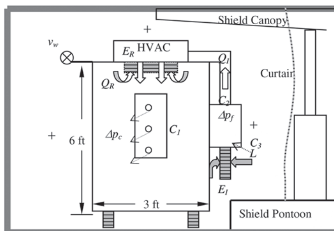
Laboratory cab test apparatus used in longwall test gallery.
