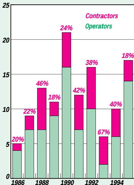
Figure 3.—Contractor and operator haulage truck fatalities and lost-time injuries, 1986–1995
