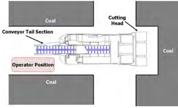
Fig. 3—Underground orientation of continuous mining machine.
