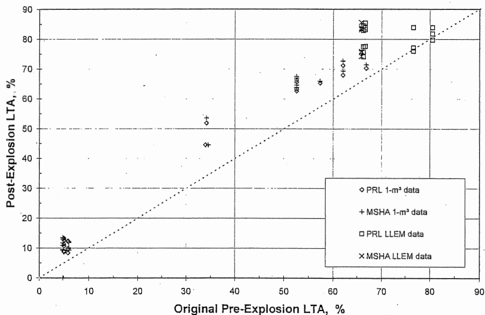
Fig. 9. Comparison of pre-explosion versus post-explosion incombustible contents from tests in the LLEM and the Fike 1-m 3 laboratory chamber.
