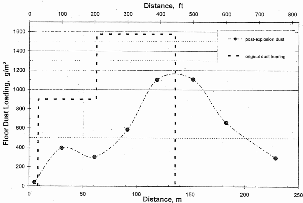
Fig. 6. Dust loading before and after explosion test #471.
