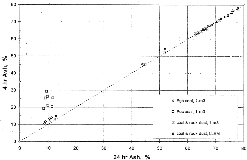
Fig. 8. Comparison of 4-hr versus 24-hr incombustible contents for post-explosion samples from tests in the Fike 1-m 3 laboratory chamber and the LLEM.
