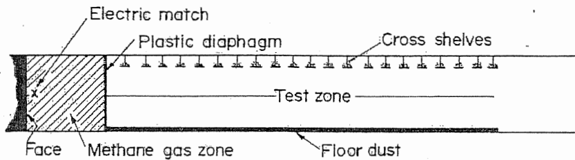
Fig. 2. Side view of D-drift in the LLEM, showing gas ignition zone and dust test zone (not to scale).
