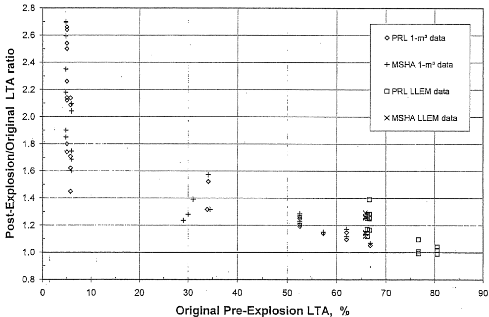
Fig. 10. Post-explosion to pre-explosion incombustible ratio from tests in the LLEM and the Fike 1-m 3 laboratory chamber.
