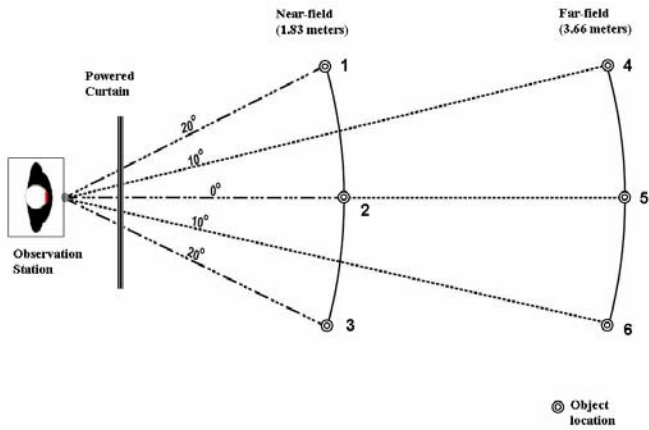
Figure 2. The experimental layout.
