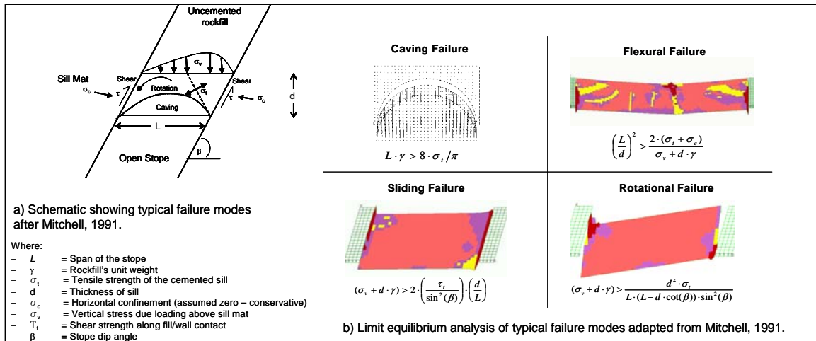
Figure 2: Limit equilibrium criteria adapted from Mitchell, 1991.
