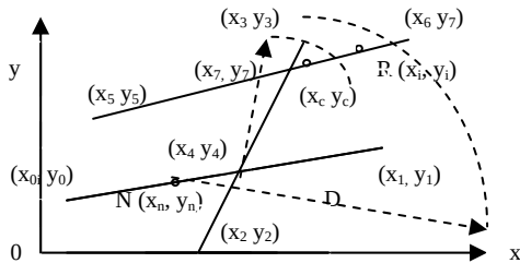
Figure 10: The second circle is drawn at (x_4, y_4) with radius D_{r-4}
