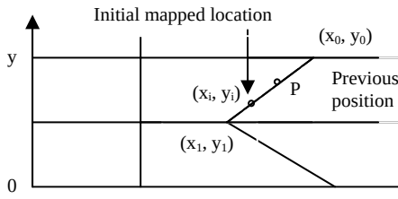
Figure 2: IML and PSP share the same line segment
