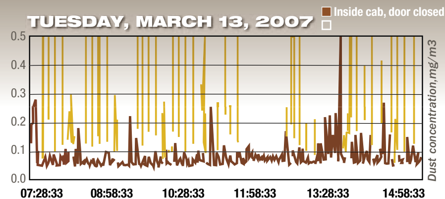
Figure 2 – Respirable-dust concentration inside enclosed cab during periods with cab door closed and open.
