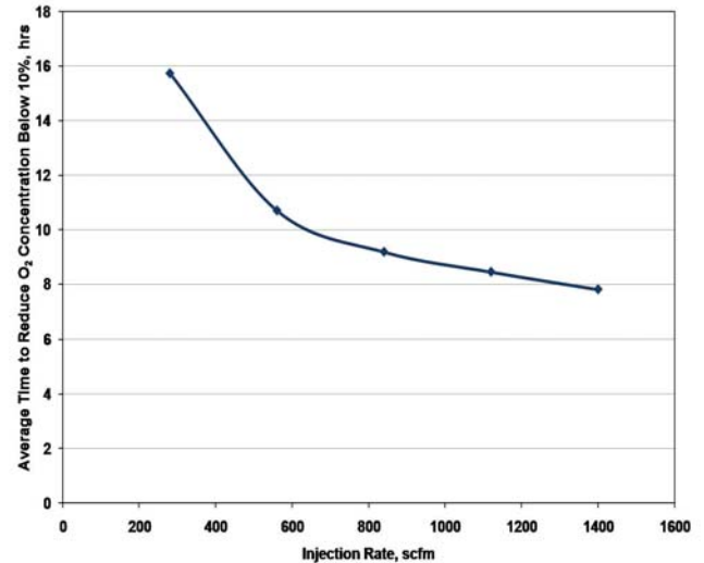
Figure 14. Time needed to reduce the O 2 level to below 10% in the simulated mine as a function of increasing the N 2 gas injection rate above the base rate used in the CFD model (280 scfm).
