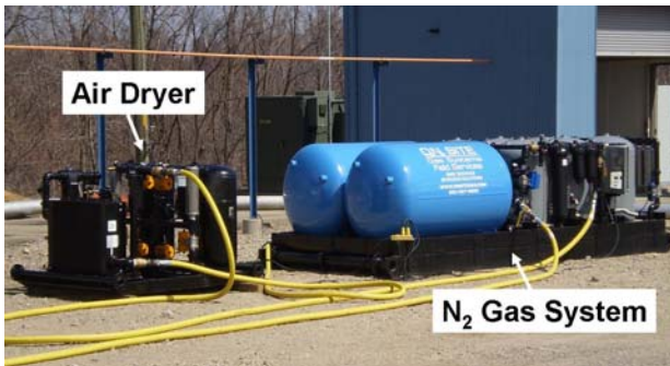
Figure 3. N 2 generating system with air dryer.
