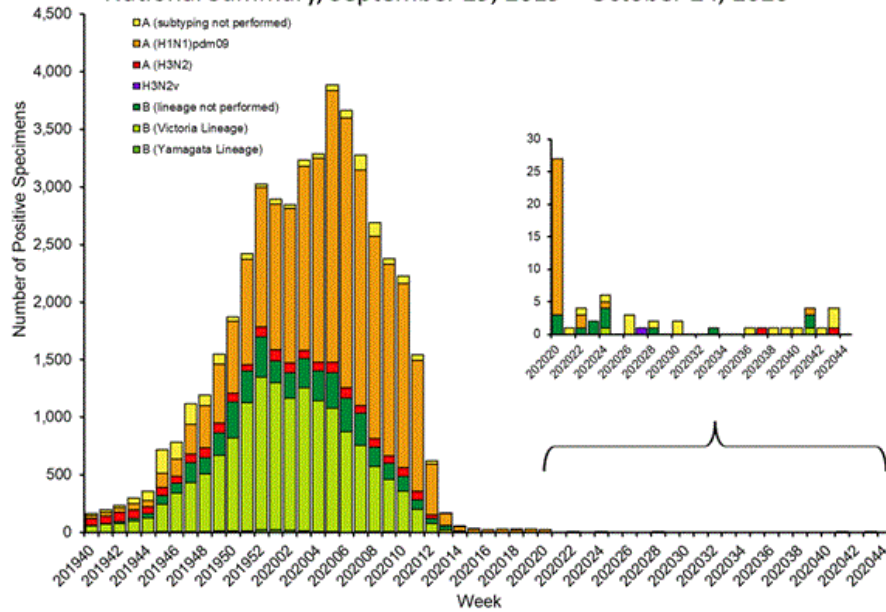
Influenza Positive Tests Reported to CDC by U.S. Public Health Laboratories, National Summary, September 29, 2019 – October 24, 2020
