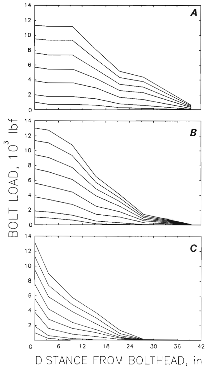
Figure A-2—Results from elastic test, mine 2. A, Bolt 1; B, bolt 2; C, bolt 3.
