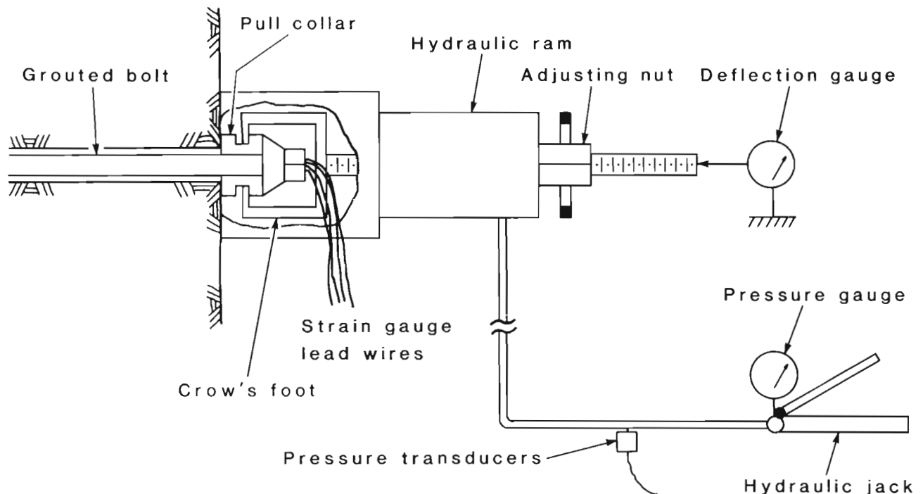
Figure 1.—Pull-test gear arrangement.
