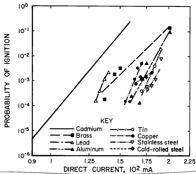
Figure 14.—Probability of ignition versus current results for 100-mH inductor circuit.
