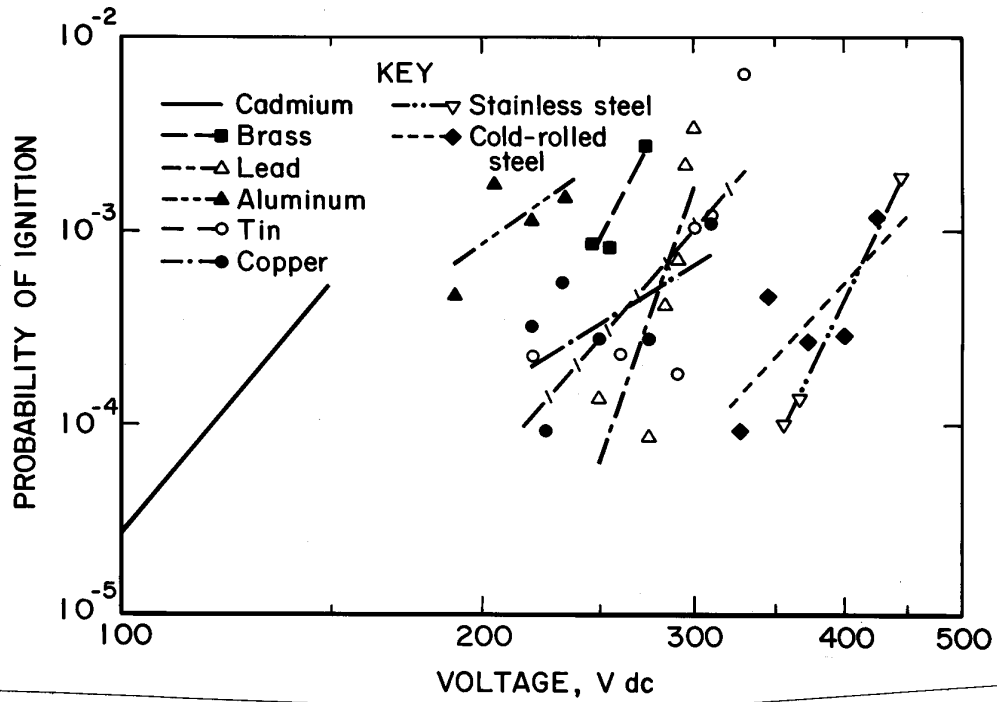
Figure 16.—Probability of ignition versus voltage results for 1.2- \mu F capacitor circuit.
