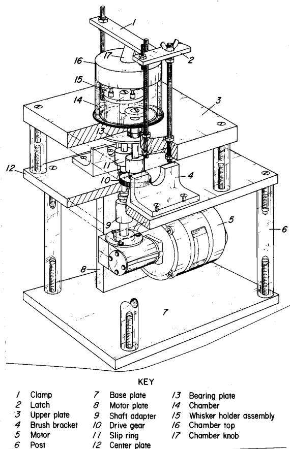
Figure 1.—Breakflash apparatus used to collect spark ignition data.
