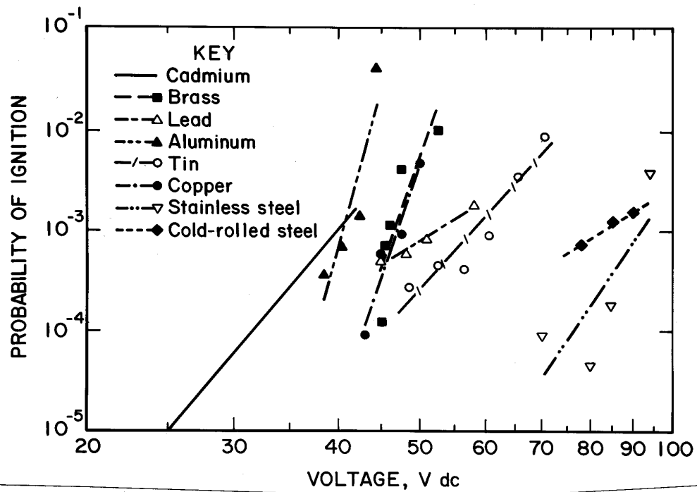
Figure 17.—Probability of ignition versus voltage results for 10.3- \mu F capacitor circuit.
