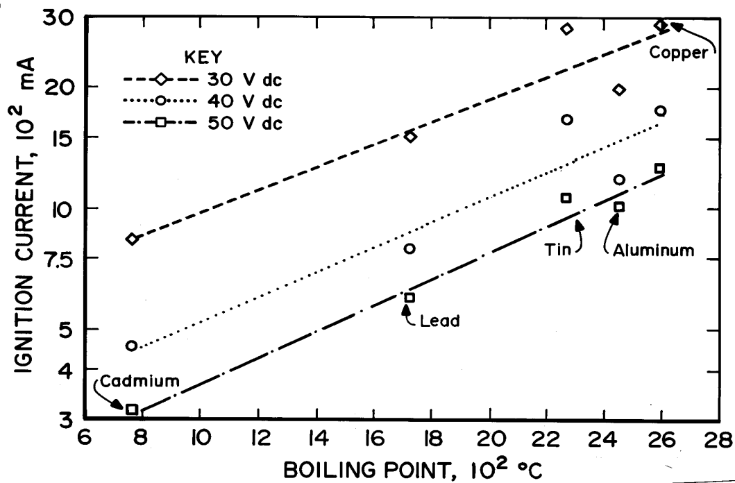
Figure 20.—Elemental disk material boiling point versus resistor circuit ignition current.
