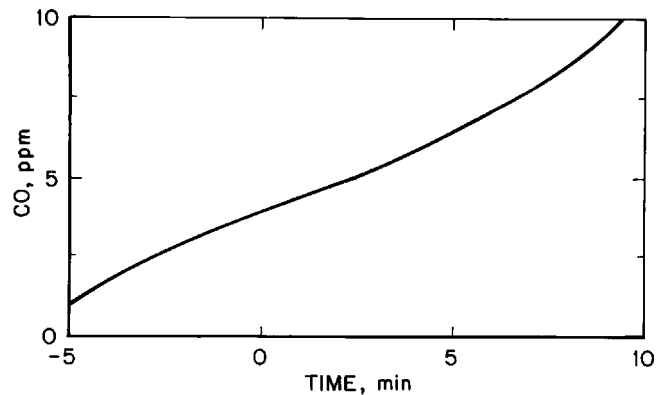
Parts per million of CO during smoldering stage at an airflow of 0.44 m/s
