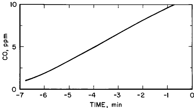
Part per million during smoldering and flaming stages at an airflow of 0.97 m/s
