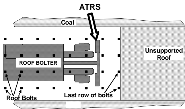
Figure 6b. Position of roof bolter after backing up so the next screen panel can be positioned on the ATRS.
