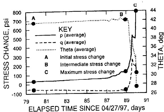
Figure 4.—Stress change in 8-Right panel
