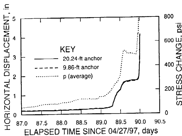
Figure 6.—Dilation and loading of 8-Right panel.
