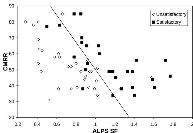
Figure 3. The ALPS case history data base and design formula, showing the effect of roof quality as measured by the CMRR.
