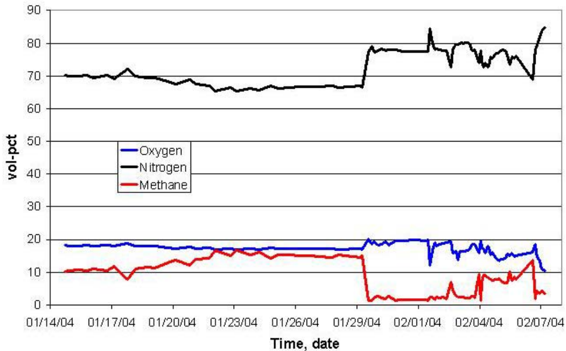
Figure 15. Gas concentrations from borehole located about 1000 feet inby the foam injection hole and about 2200 feet inby the remote seal.
