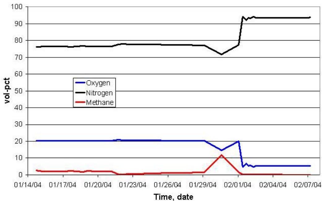
Figure 14. Gas concentrations for the foam injection location, approximately 1200 feet inby the remote seal.
