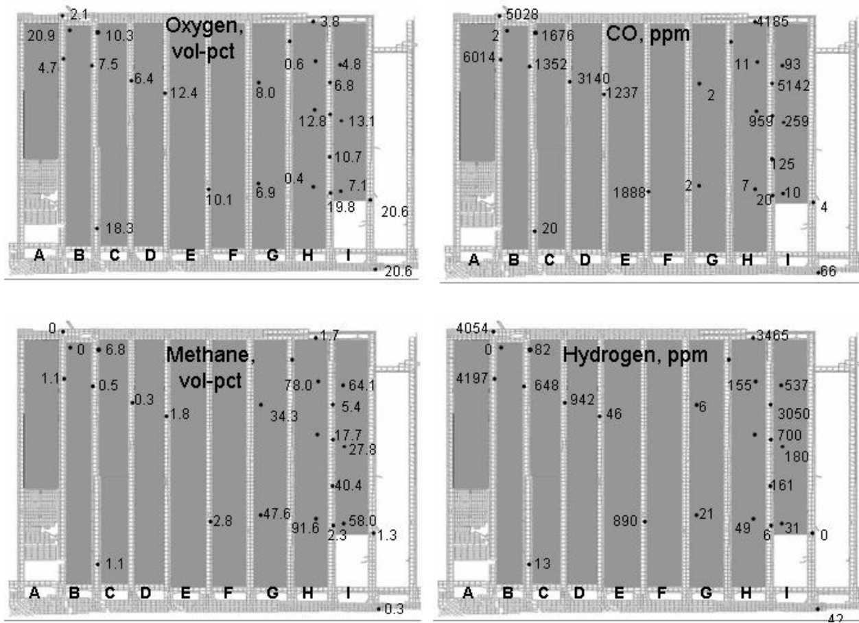
Figure 4. Gas concentrations at various locations in longwall district 8 on October 6, 2003.
