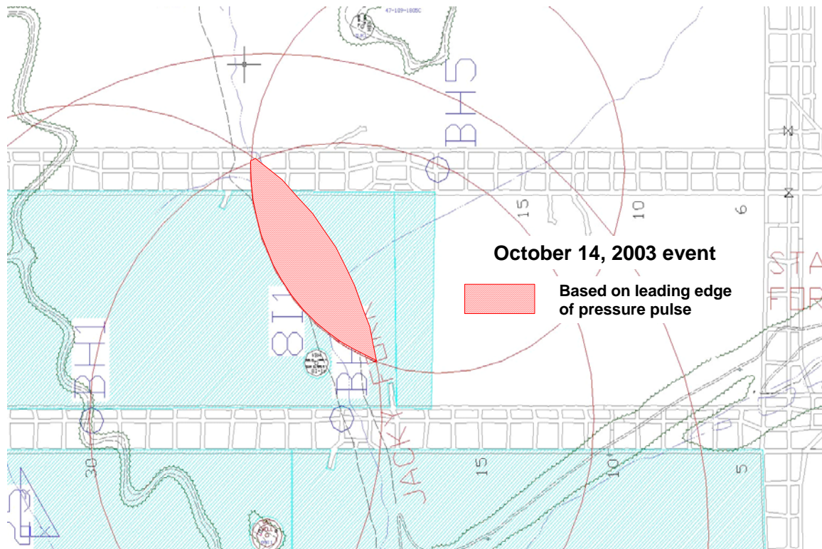
Figure 7. Probability space of location of ignition source on October 14, 2003 based on leading edge triangulation method.
