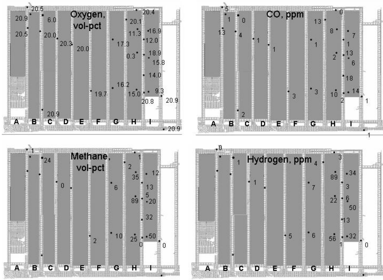
Figure 2. Gas concentrations at various locations in longwall district 8 on September 30, 2003.
