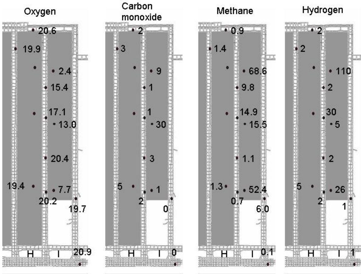
Figure 8. Gas concentrations for panels 8H and 8I on January 26, 2004.
