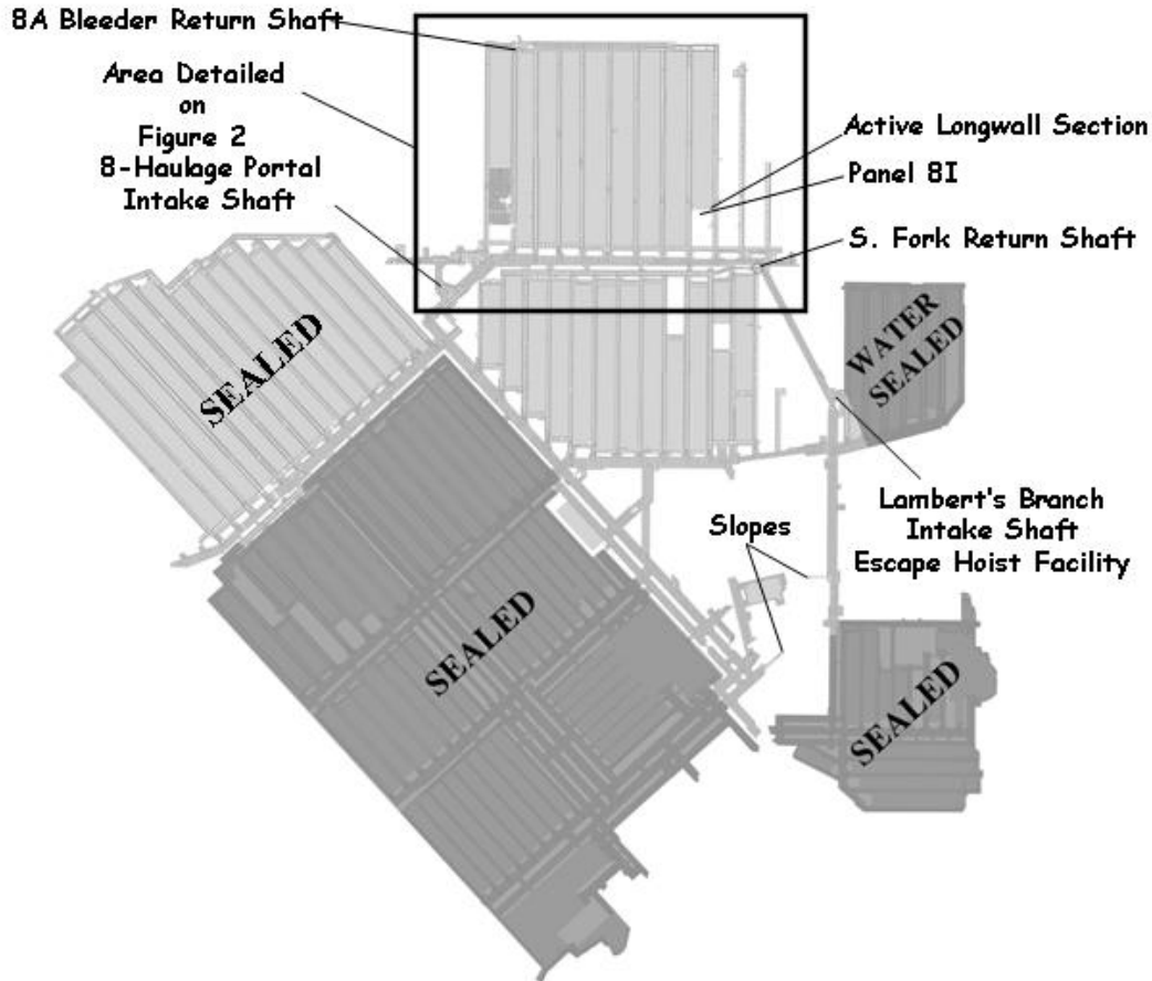
Figure 1. Schematic of the Pinnacle Mine.
