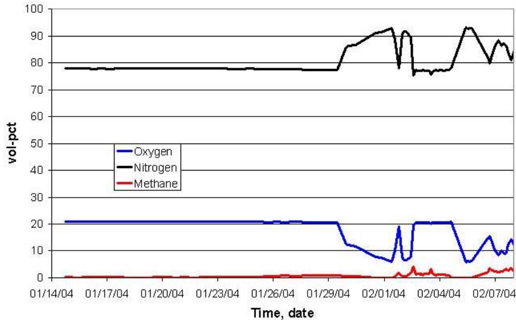
Figure 13. Gas concentrations from Jan 14 to February 7 at a borehole just inby the location of the remotely-installed seal.
