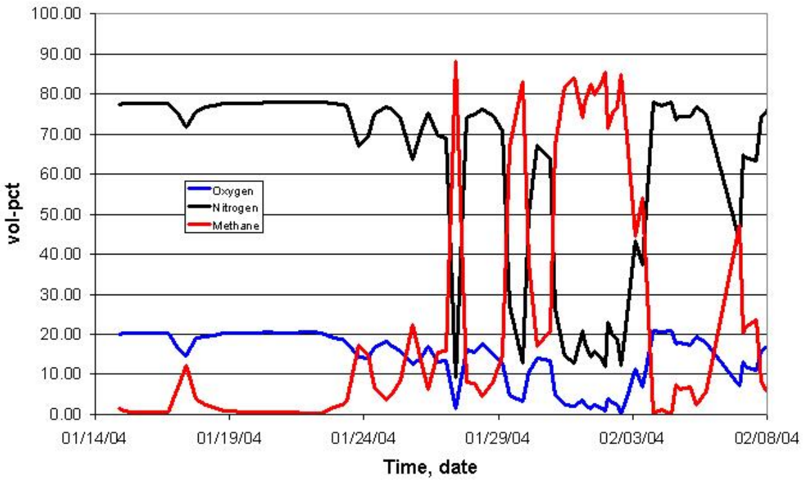
Figure 18. Gas concentrations from borehole in the caved area near the tailgate entries.
