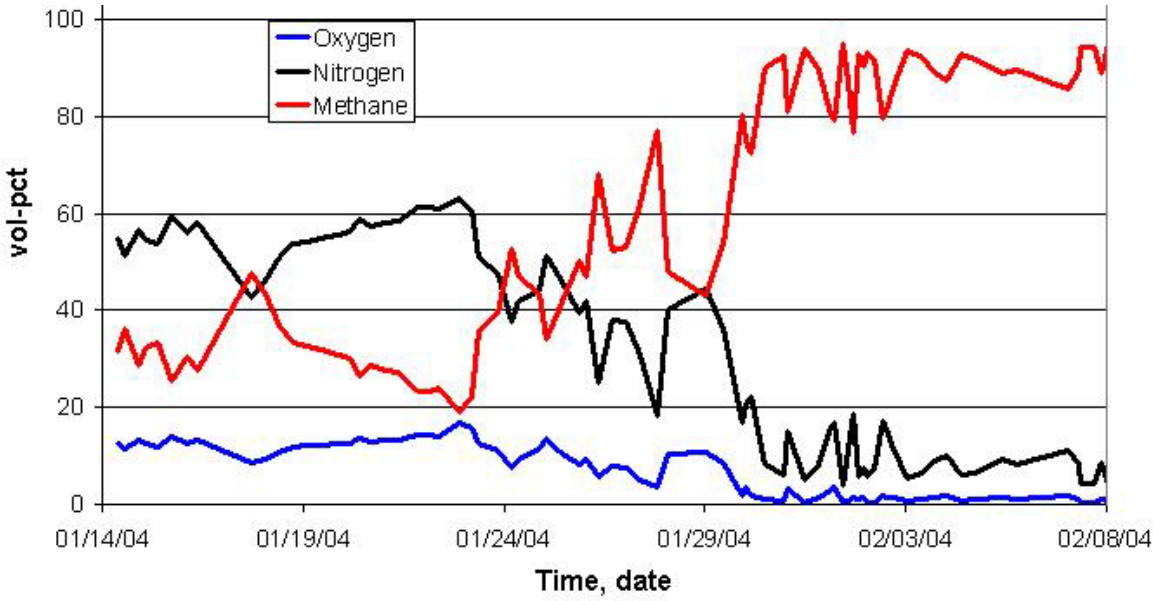
Figure 17. Gas concentrations at a location behind the longwall face near the tailgate entries.
