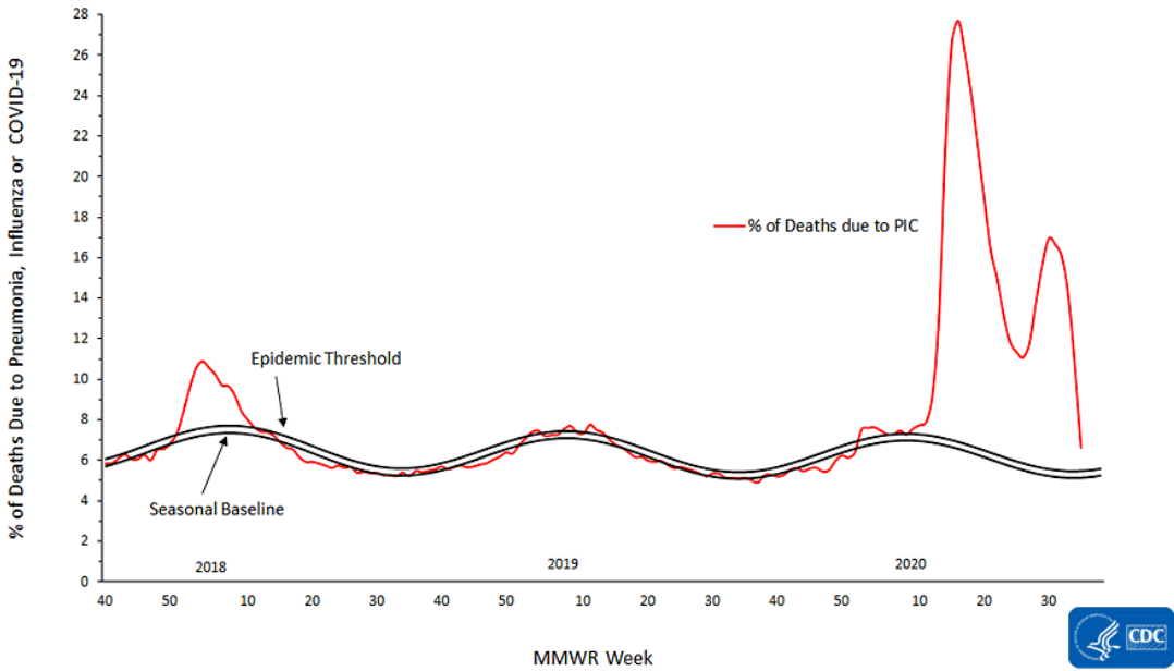
NCHS Mortality Reporting System: Pneumonia, Influenza and COVID-19 Mortality Data through the week ending August 29, 2020, as of September 3, 2020
