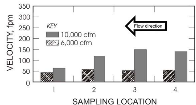
Figure 14. Thirty-five ft curtain setback, 13-ft-wide entry.
