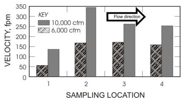
Figure 13. Twenty-five ft curtain setback, 16 ½-ft-wide entry.
