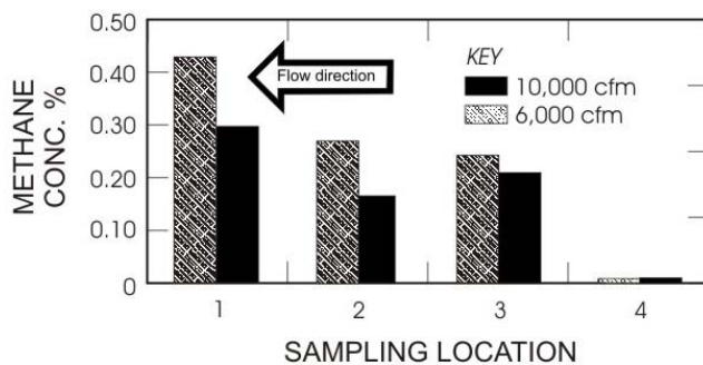
Figure 16. Methane concentrations, 25-ft curtain setback, 13-ft entry.
