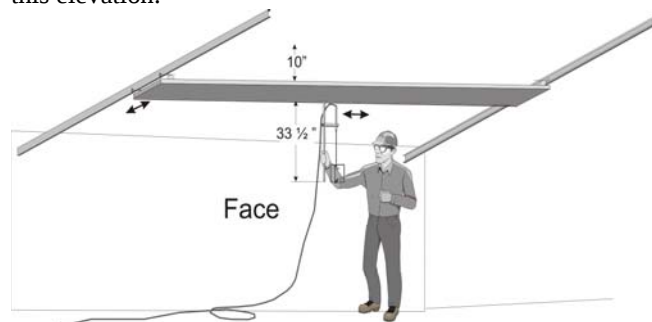
Figure 4. Overhead support system.
