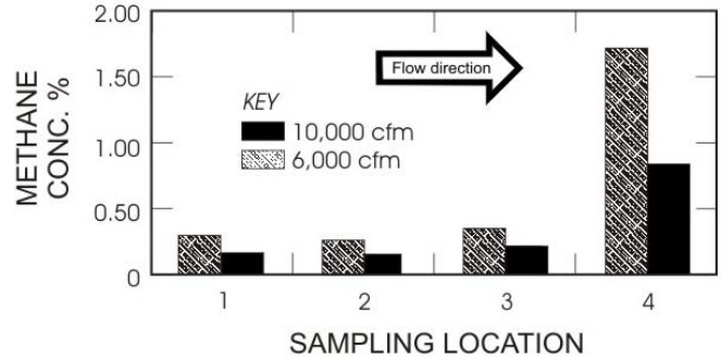
Figure 17. Methane concentration, 25-ft curtain setback, 16 ½-ft entry.
