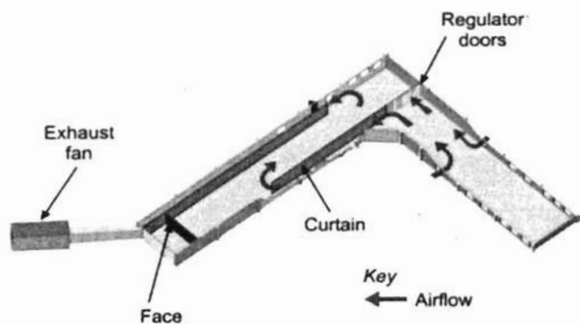
Figure 1 — Ventilation Test Gallery.
