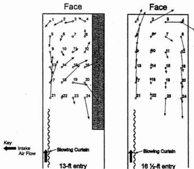
Figure 6 — Flow diagrams for 7.6-m (25-ft) setback.
