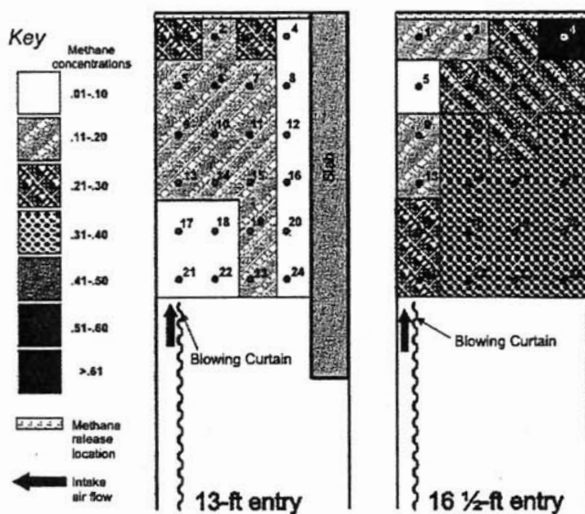
Figure 9 — Methane distribution for 7.6-m (25-ft) setback, 4.7 m 3 /s (10,000 cfm) intake.
