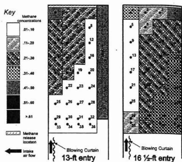
Figure 10 — Methane distribution for 10.7-m (35-ft) setback, 4.7 m 3 /s (10,000 cfm) intake.
