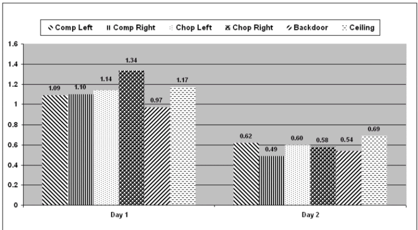
Figure 5 - Respirable dust concentrations in mg/m 3 for filters that had been in operation for 3-4 months (day 1) and new filters (day 2) on six air cleaning units.
