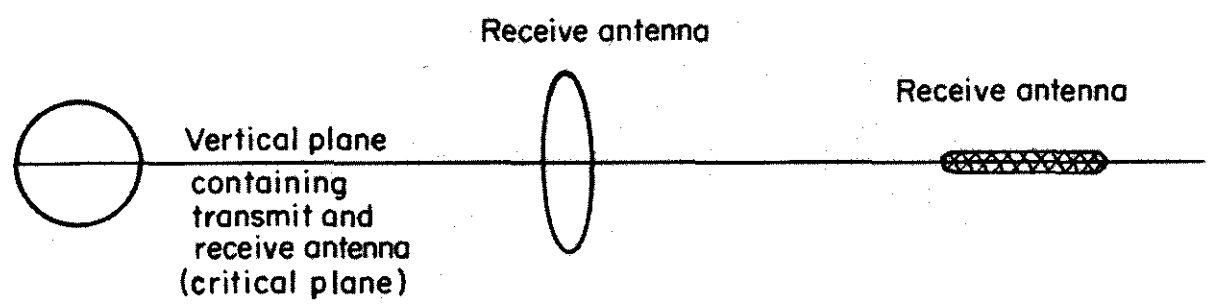
FIGURE 5: - Determining "critical planes."
