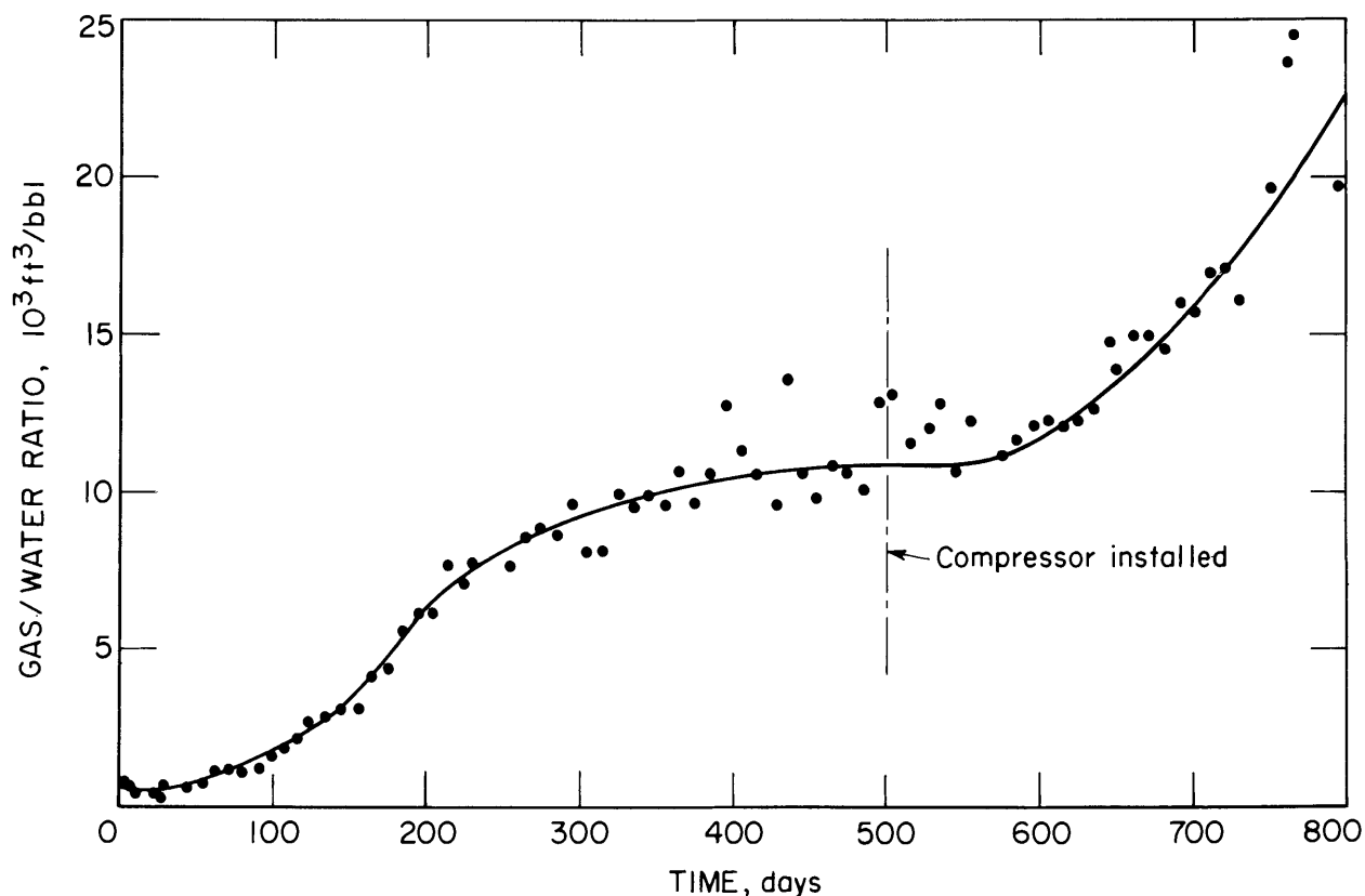
FIGURE 12. - Gas-water ratio from Fields large-diameter multipurpose borehole (4).
