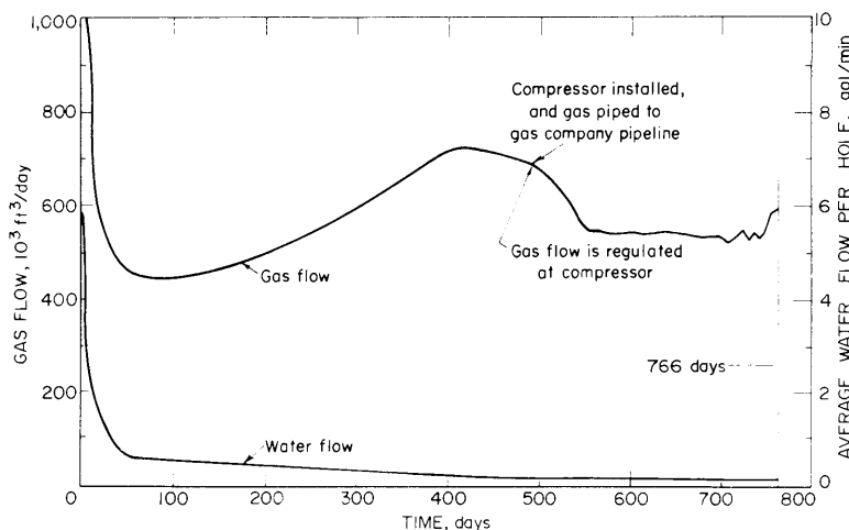
FIGURE 4. - Gas and water flow rates for the large-diameter borehole (4).
