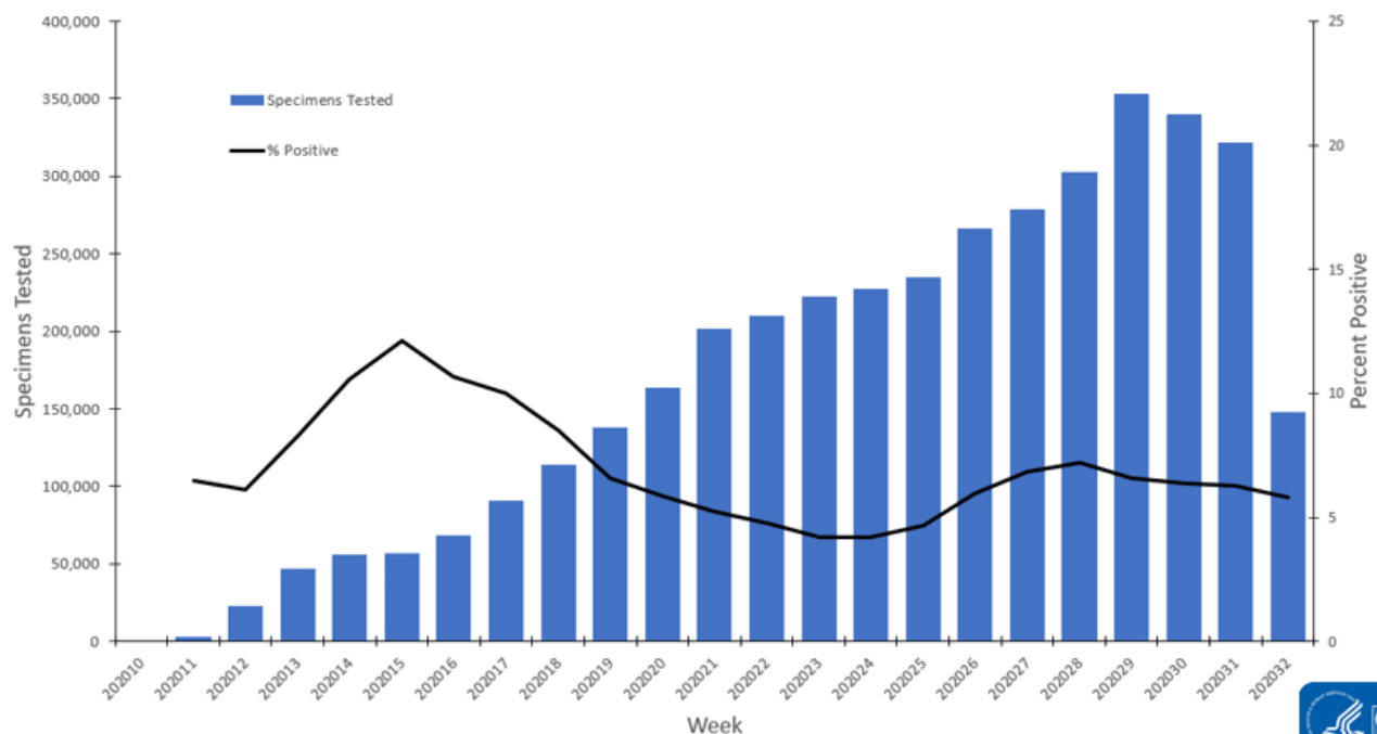
U.S. Clinical Laboratories Reporting to the National Respiratory and Enteric Virus Surveillance System: Number of Specimens Tested and Percent Positive for SARS-CoV-2 March 8, 2020 – August 8, 2020
