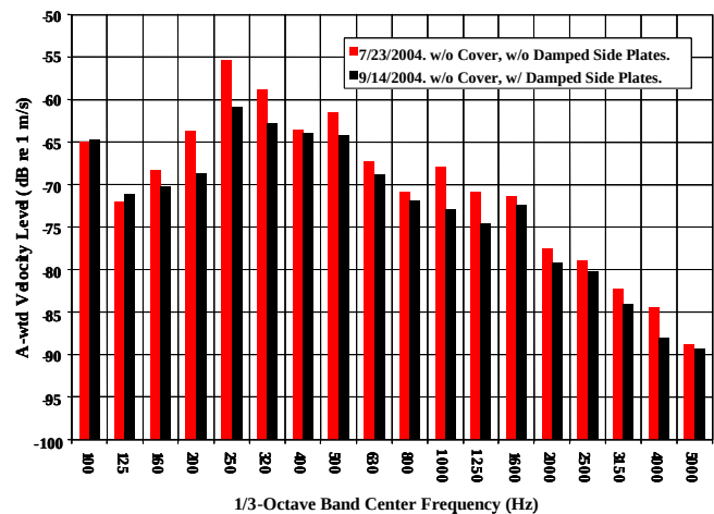
Figure 24. A-weighted average velocity on right side of the screen without and with damped sides.
