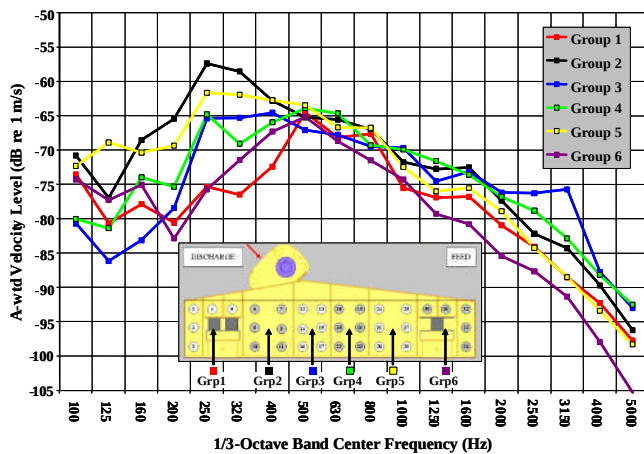
Figure 20. A-weighted surface-averaged velocity levels.
