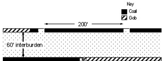
Figure 10. Cross-section showing panel geometry at the time of a large face bump at Utah Mine A.
