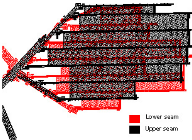
Figure 9. Layout of yield pillar longwall panels at Utah Mine A.
