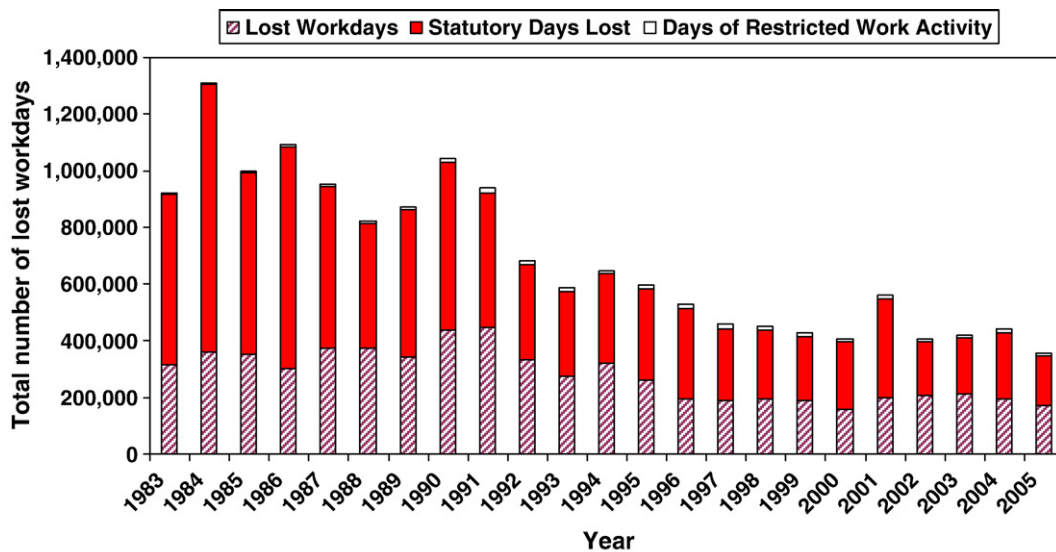
Fig. 2. Lost Workdays for Nonfatal Injuries - Coal Mine Operators.
