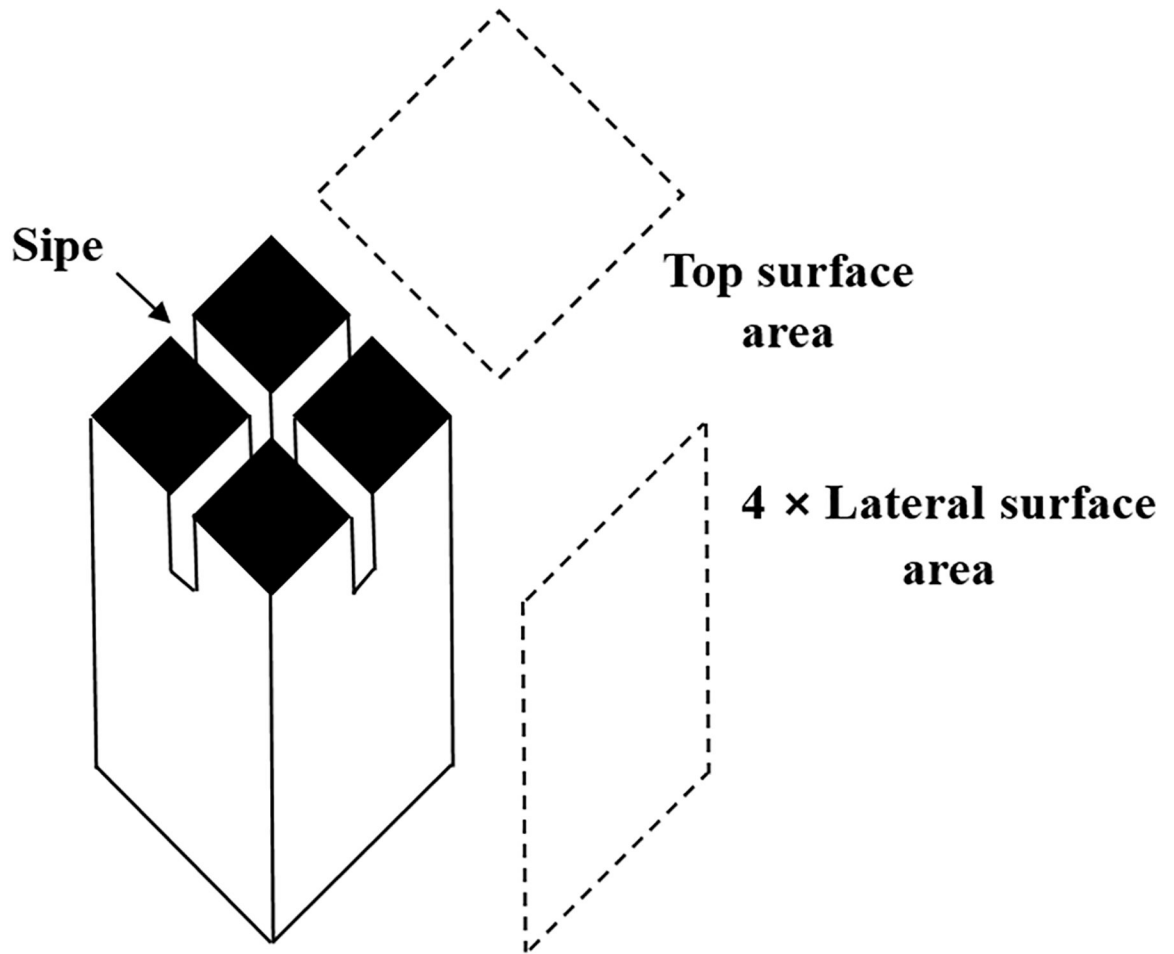
Figure 2. Shape factor measurement of a tread (black region represents tread surface area)
