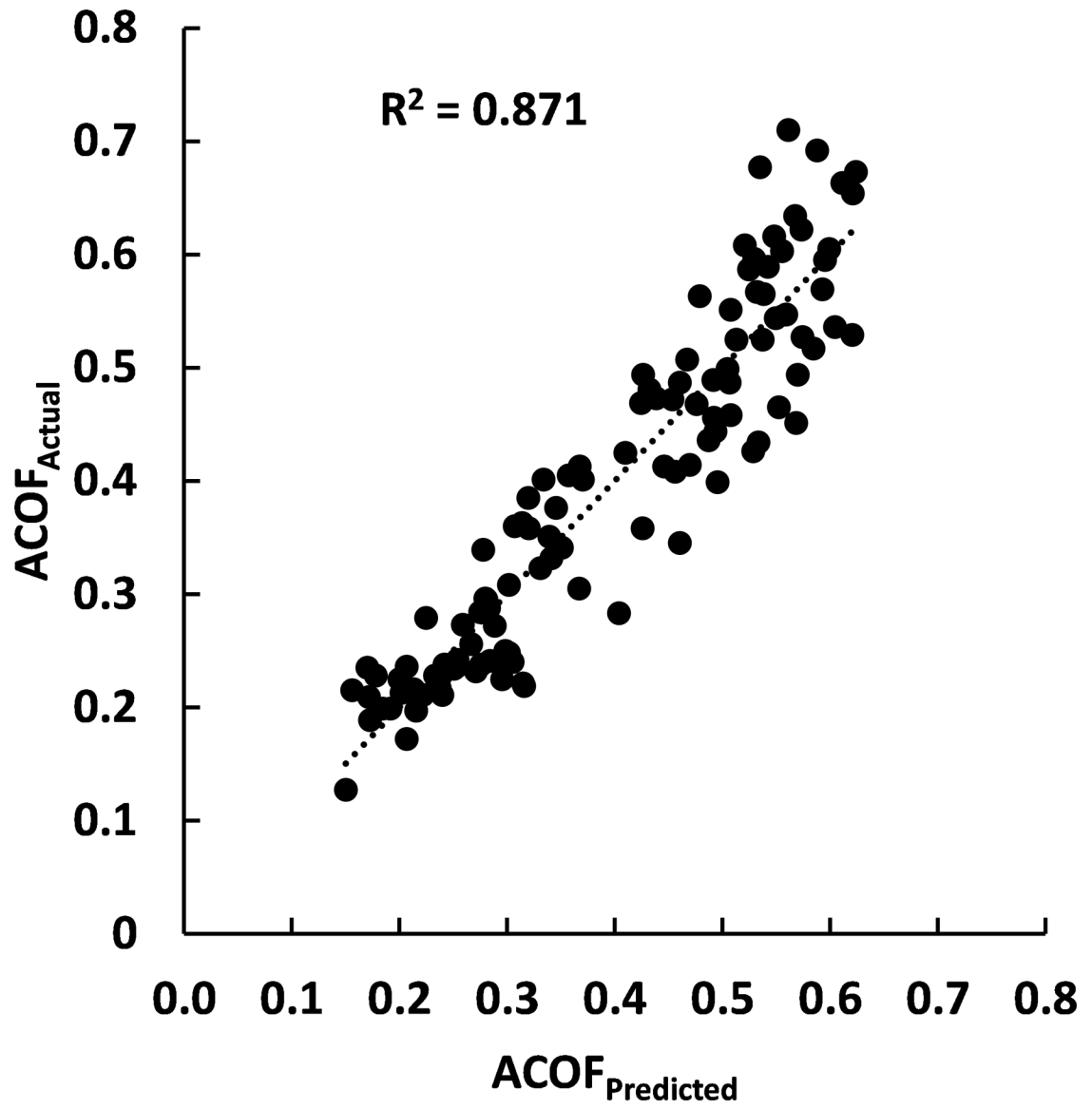
Figure 6. Actual vs. predicted ACOF (response variable) from the forward model (Eq. 4).
