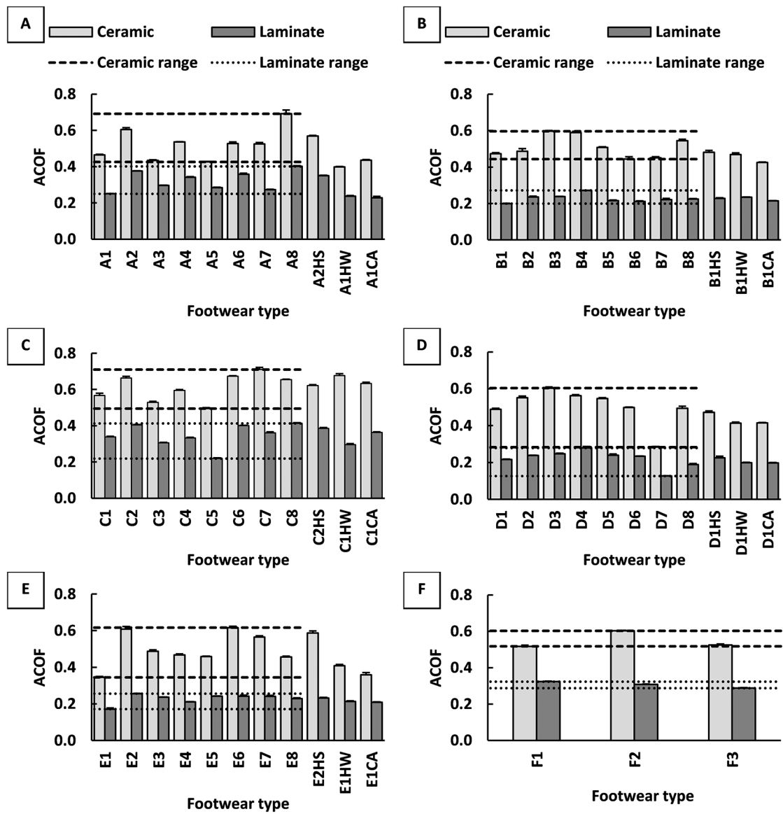
Figure 4. ACOF for ceramic (light grey) and laminate (dark grey) tile with canola oil for the shoe brands: (A) Shoes for Crews, (B) Tredsafe, (C) SR Max, (D) safeTstep, (e) Dr. Scholl's, and (F) Timberland PRO. The dashed lines and round dots on each plot show the range of ACOF within brands (for unmodified shoes) on both ceramic and laminate tile, respectively.
