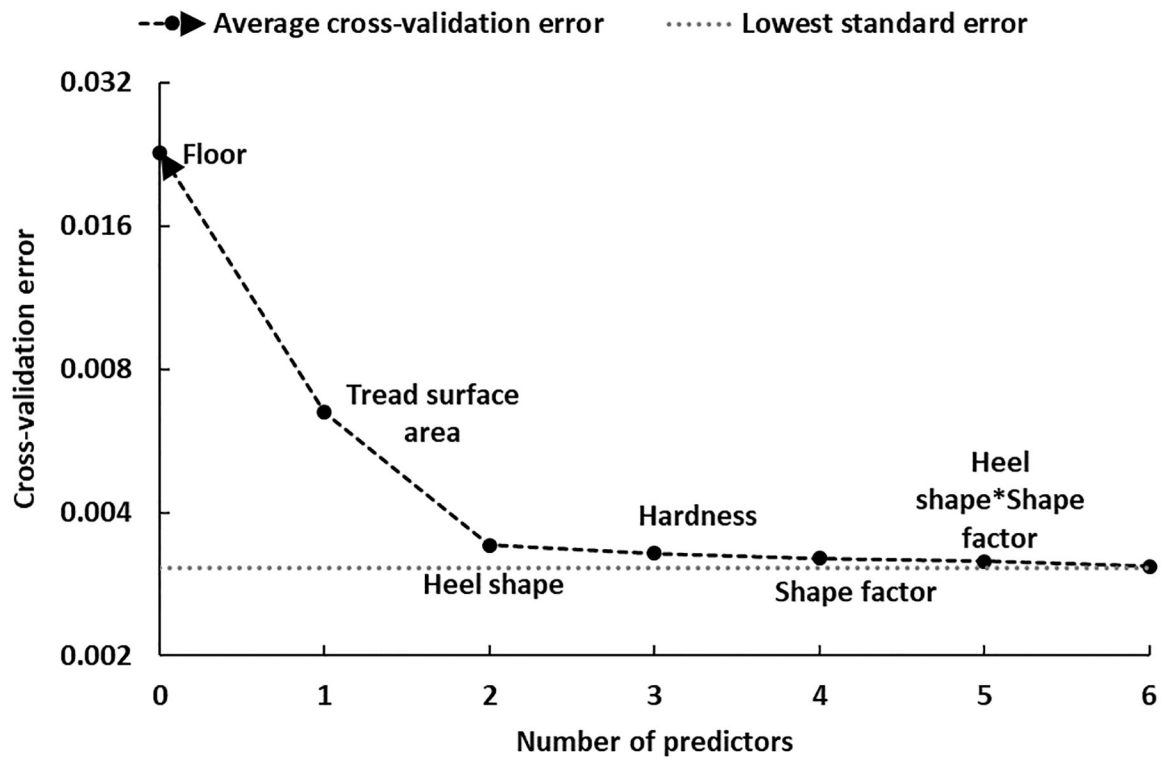
Figure 5. Cross-validation error for different number of significant predictors in the reduced models. The data label above/below each data point indicates which parameter was removed during backward elimination. Standard error for each data point is small, which is not visible on the plot.
