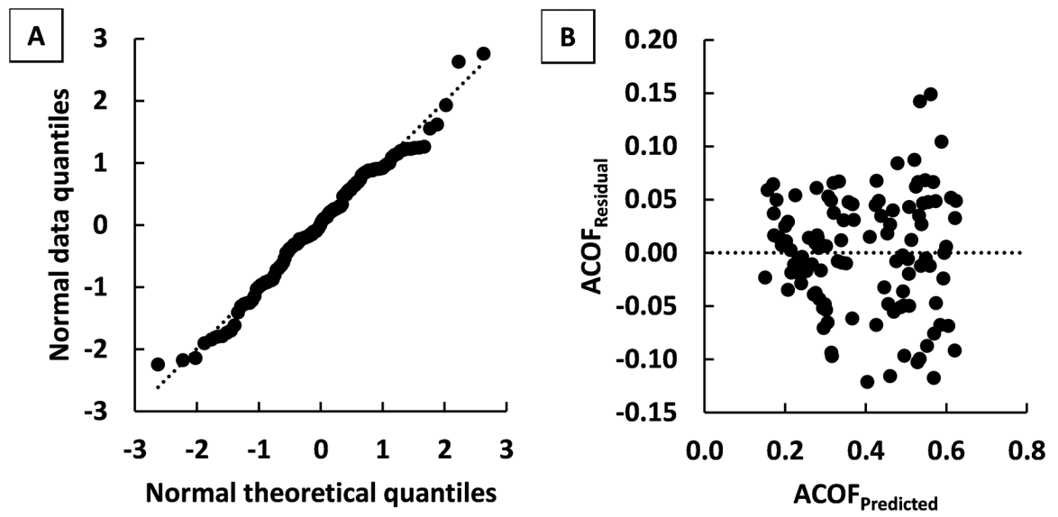
Figure 7. Residual analysis performed on the forward model: (A) normal quantile plot to assess the assumption of normality; and (B) plot of residual vs. predicted ACOF to assess assumption of homoscedasticity.
