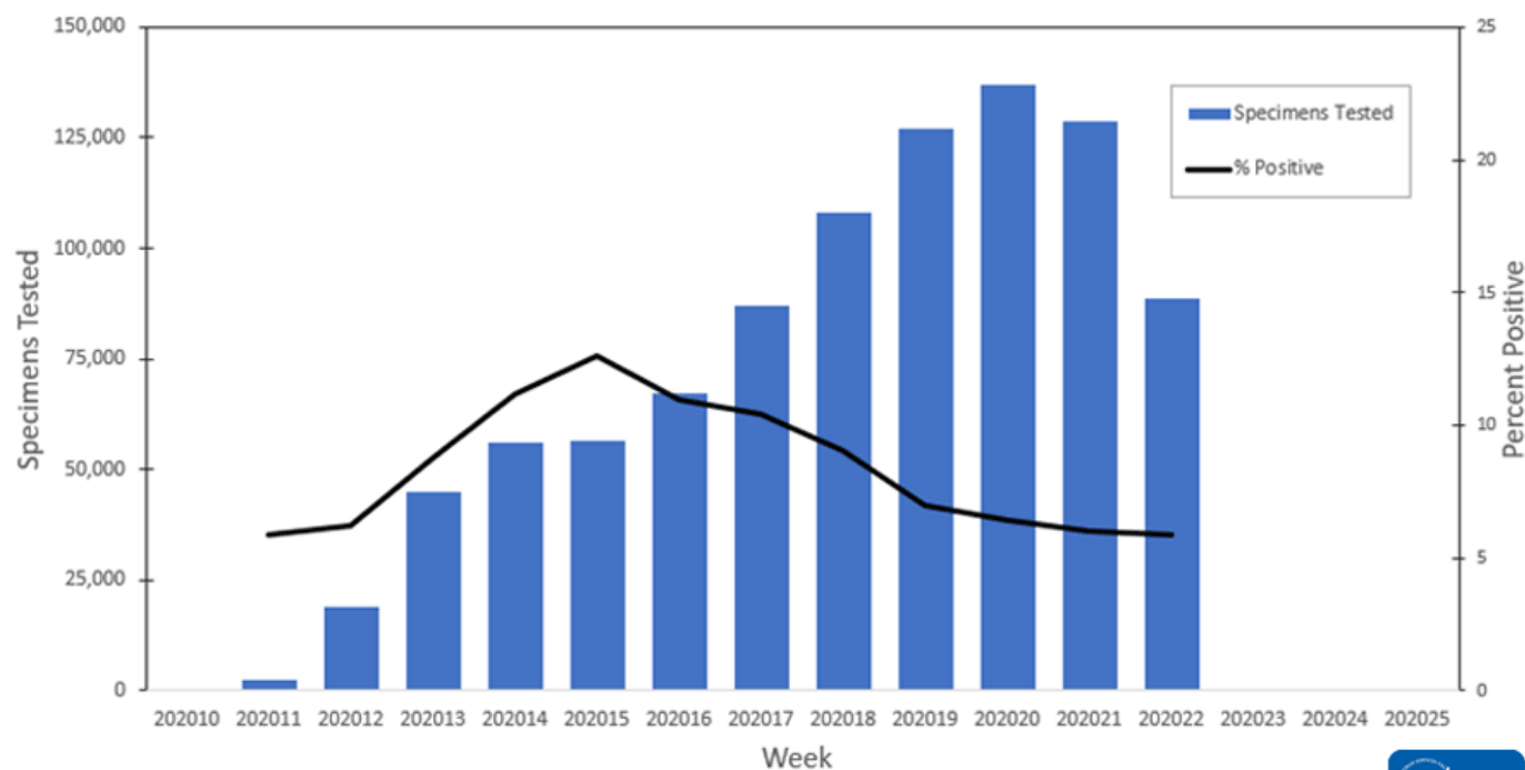
U.S. Clinical Laboratories Reporting to the National Respiratory and Enteric Virus Surveillance System: Number of Specimens Tested and Percent Positive for SARS-CoV-2 March 8, 2020 - May 30, 2020
