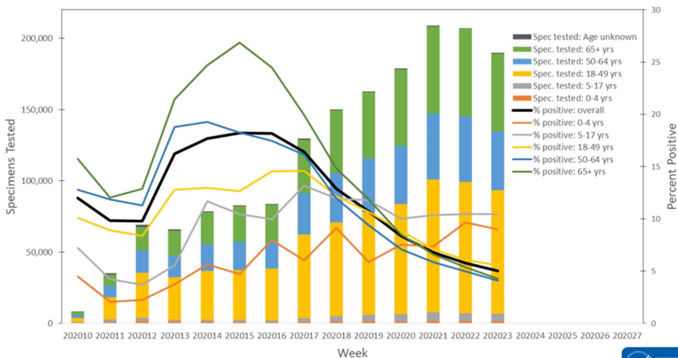
U.S. State and Local Public Health Laboratories Reporting to CDC: Number of Specimens Tested and Percent Positive for SARS-CoV-2 March 1, 2020 – June 6, 2020
