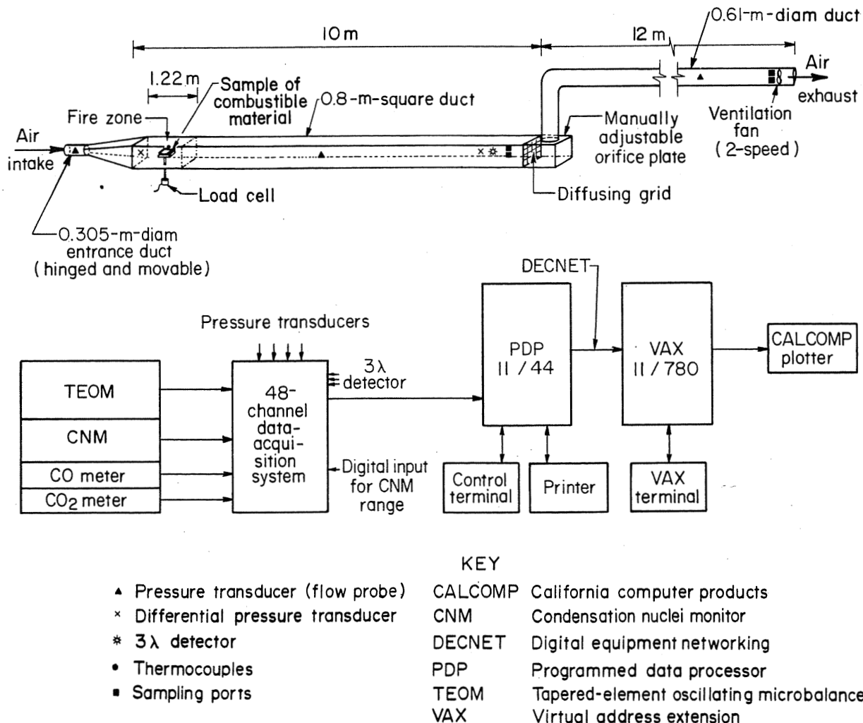
Figure 2.—Schematic of Intermediate-scale fire tunnel (top) and data-acquisition system (bottom).
