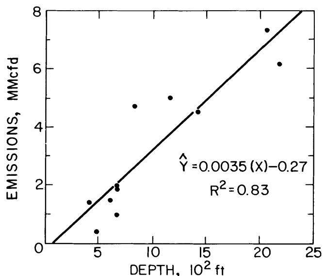
FIGURE 5. - Emissions versus depth of coal. ( \hat{Y} = estimated emissions; X = depth; R^2 = coefficient of determination.)
