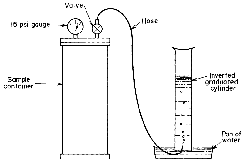
FIGURE 6. - Apparatus used to measure gas emission from a coal sample.
