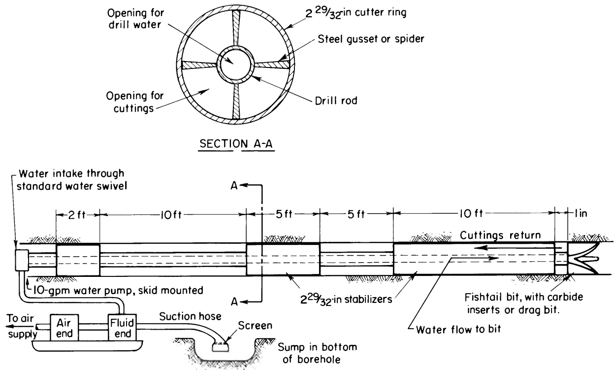
FIGURE 7. - Stabilizer assembly.
