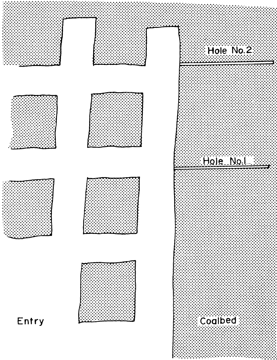
FIGURE 1. - Plan view—coal mine entry with two boreholes.
