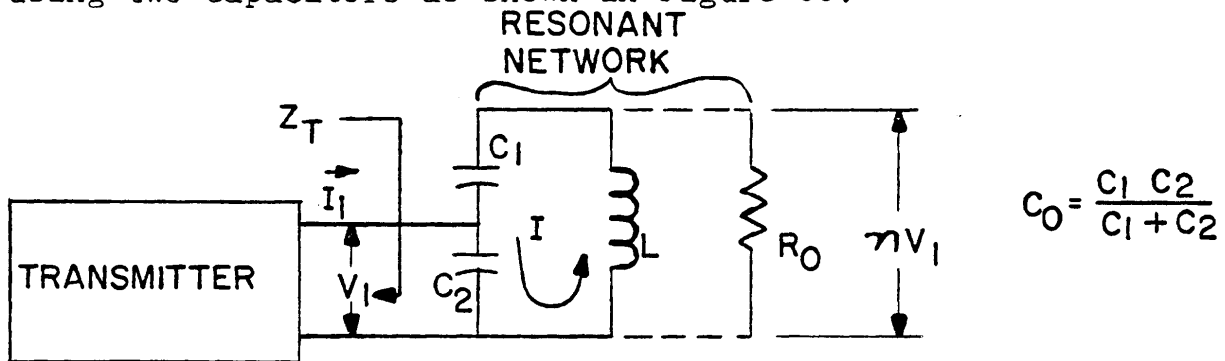
FIGURE 35. TYPICAL MATCHING NETWORK
