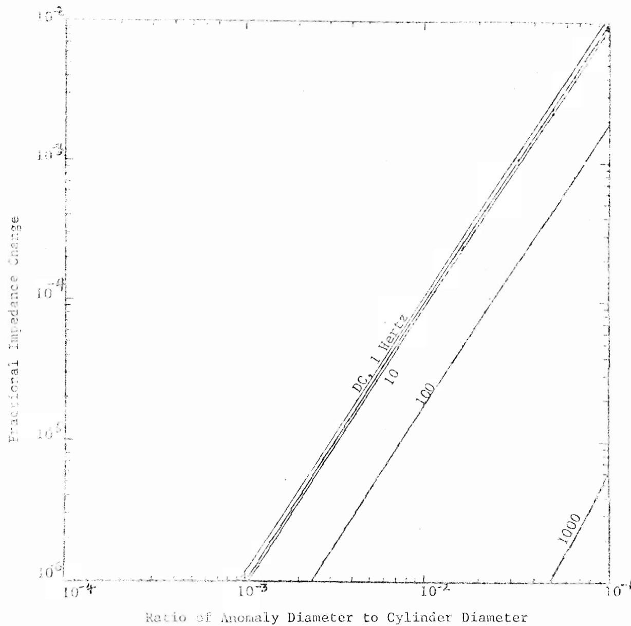
Figure 5 : Fractional Impedance Change for a Sensor as a Function of Anomaly Size. The Anomaly is Offset one-half the Cylinder Radius ( \rho_i = .5a ).
