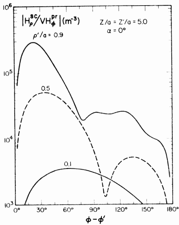
Fig. 2. The normalized magnitude of the scattered radial magnetic field for various void locations \rho' .
