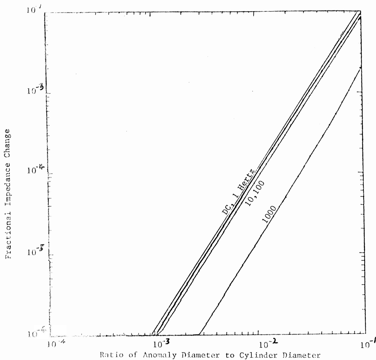
Figure 6 : Fractional Impedance Change for a Sensor as a Function of Anomaly Size. The Anomaly is Near the Cylinder Surface. ( \rho_i = .8a )
