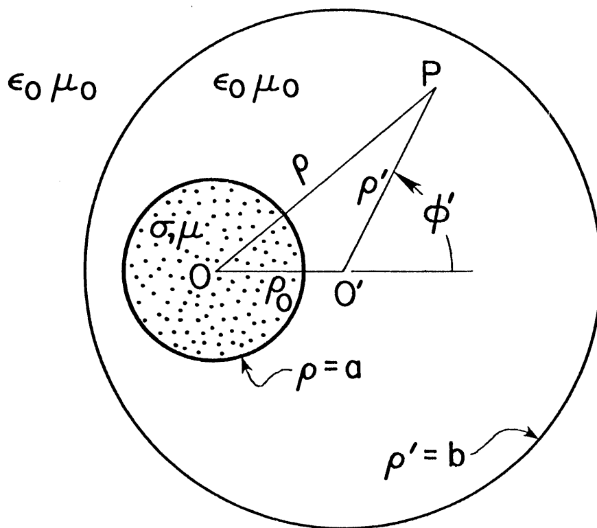
Fig. 12. Cross-section view of the non-concentrically located sample.
