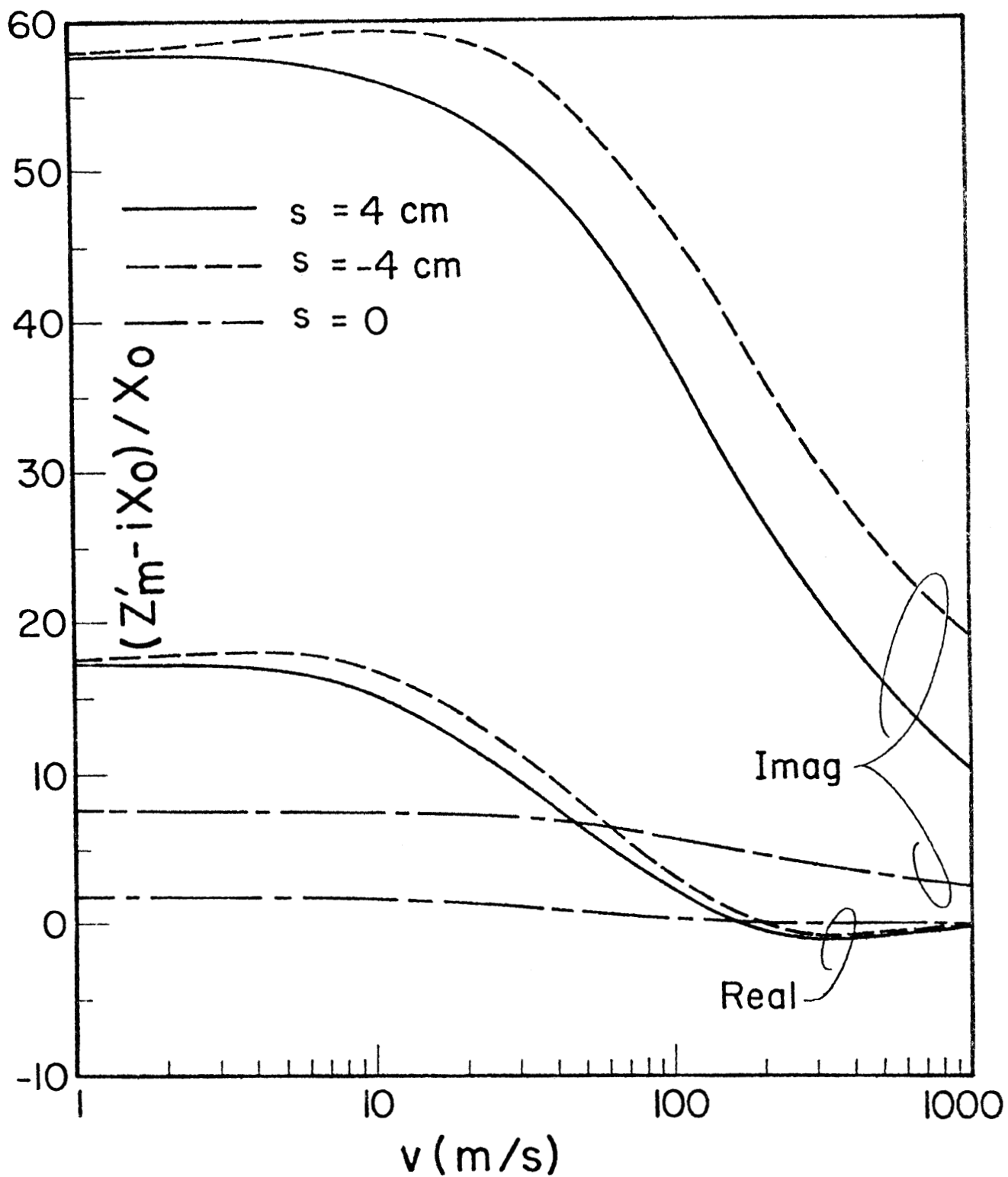
Fig. 13. Normalized response for coaxial sensor a function of v for f = 10 Hz, \sigma = 10^6 mho/m and \mu/\mu_0 = 200 , s = 0, -4 and +4 cm.
