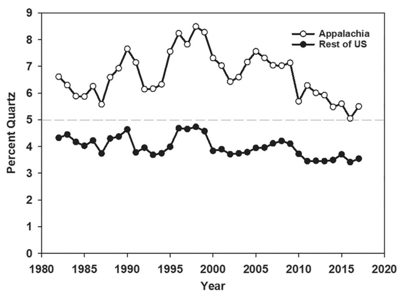
FIGURE 4. Mean percent quartz in samples for central Appalachia (MSHA Districts 4, 5, and 12 combined) and the rest of the United States (MSHA Districts 2–3, 7–10 combined) by year. MSHA, Mine Safety and Health Administration
