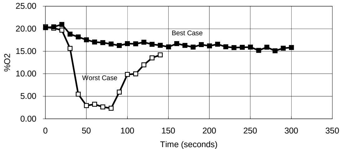
Figure 6. The measured O 2 concentrations for the best and worst sample materials as a function of time from ignition of the gas burner.
