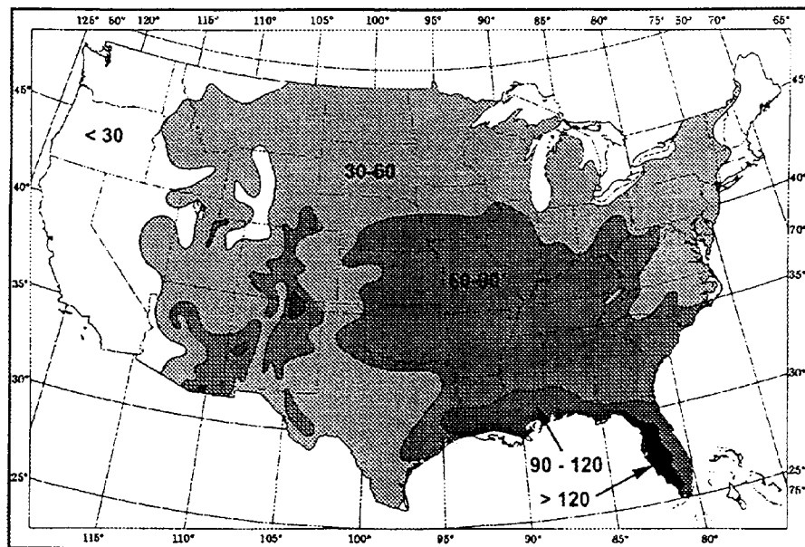
Figure 2. Average number of thunderstorms per year based on thunder reports from weather observers (from M.J. Changerv. 1981).
