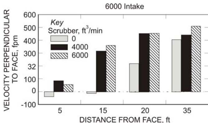
Figure 11. Left side airflow perpendicular to face (6000 ft 3 /min intake).
