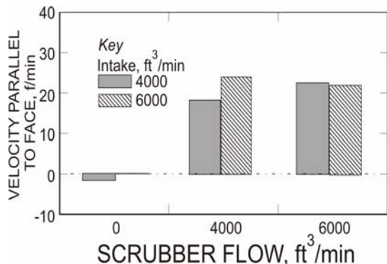
Figure 7. Airflow parallel to face (Location 2).
