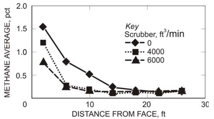
Figure 16. Methane concentration with distance from face (6000 ft 3 /min intake).
