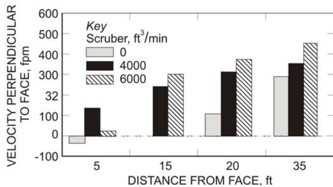
Figure 10. Left side airflow perpendicular to face (4000 ft 3 /min intake).
