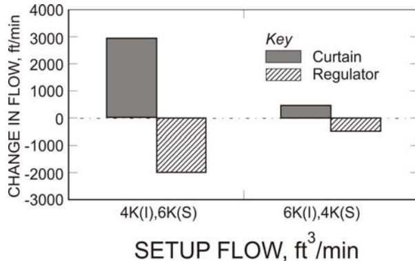
Figure 12. Airflow changes measured behind the curtain and at the regulator door due to scrubber use.
