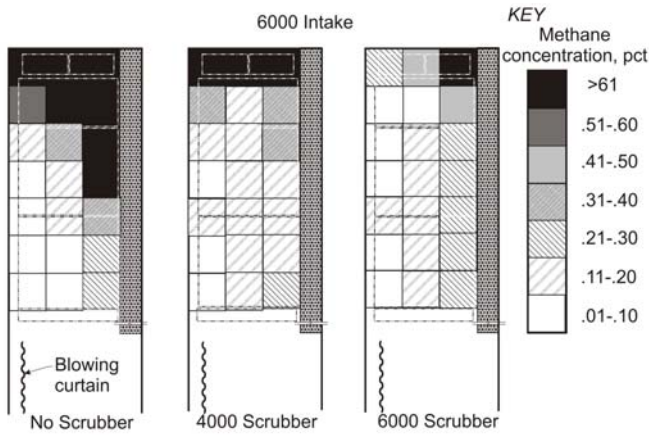
Figure 14. Methane concentrations above mining machine (6000 ft 3 /min intake flow).
