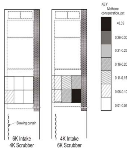
Figure 17. Methane from scrubber exhaust.
