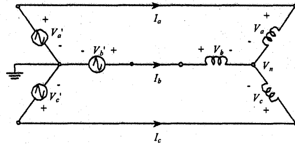
Figure 1. Wye-connected power source and induction motor.
