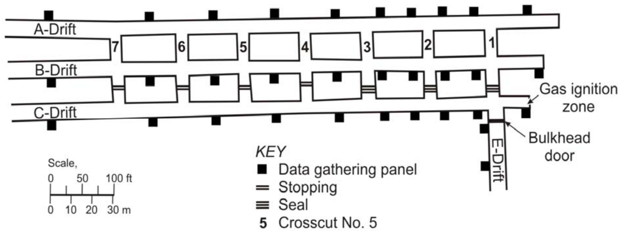
Figure 1. Plan view of the Lake Lynn Experimental Mine showing multiple entry area and stopping locations
