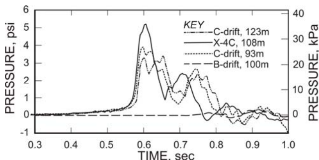
Figure 4. Pressure traces for the block stopping in X-4 during LLEM test #428
