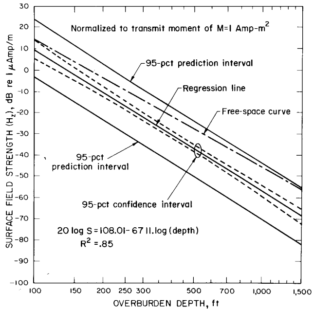
Fig. 2. Uplink regression results for 1050-Hz-normalized vertical signal strength vs. depth.
