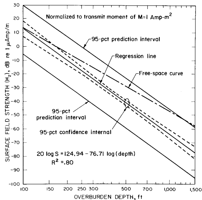
Fig. 4. Uplink regression results for 3030-Hz-normalized vertical signal strength vs. depth.
