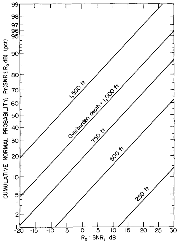
Fig. 13. Cumulative probability distribution of SNR expected above United States underground coal mines at 1950 Hz.
