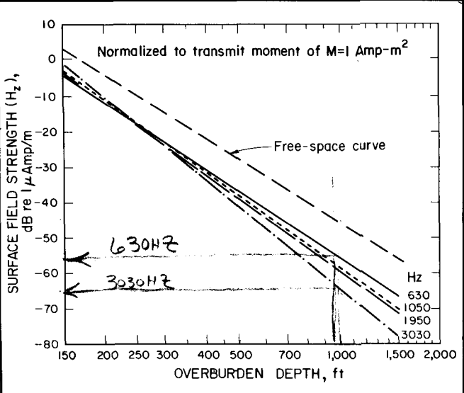
Fig. 5. Normalized overburden response curves—uplink regression results: Average surface vertical signal strength vs. overburden depth by frequency.
