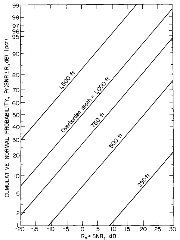
Fig. 12. Cumulative probability distribution of SNR expected above United States underground coal mines at 1050 Hz.
