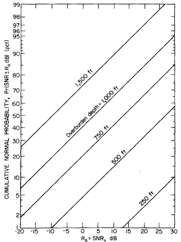
Fig. 14. Cumulative probability distribution of SNR expected above United States underground coal mines at 3030 Hz.
