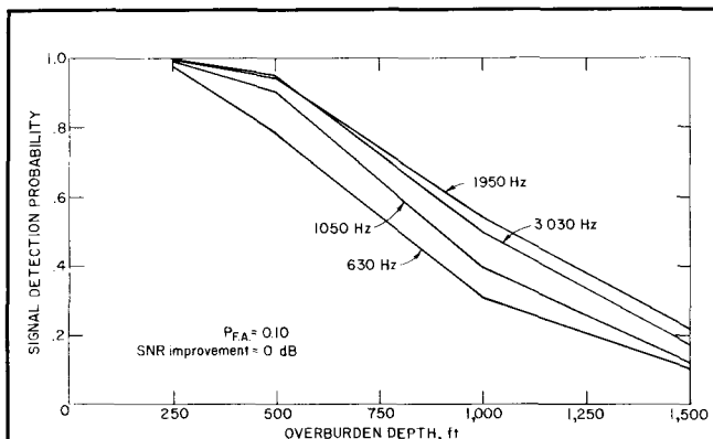
Fig. 17. Predicted probability of signal detection vs. overburden depth by frequency for the GI transmitter as found by the ROC method.
