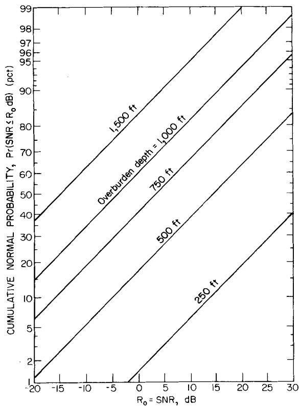
Fig. 11. Cumulative probability distribution of SNR expected above United States underground coal mines at 630 Hz.
