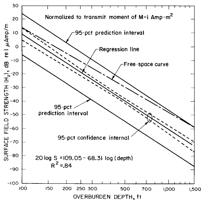
Fig. 3. Uplink regression results for 1950-Hz-normalized vertical signal strength vs. depth.
