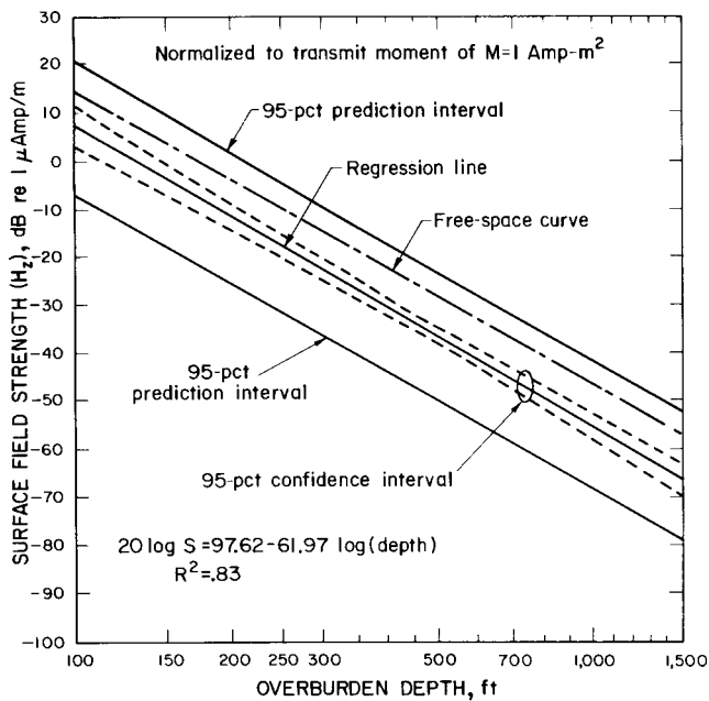
Fig. 1. Uplink regression results for 630-Hz-normalized vertical signal strength vs. depth.
