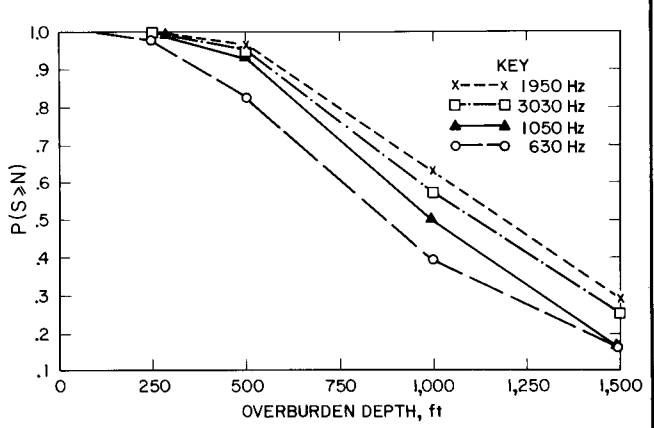
Fig. 15. Probability that mean rms signal is greater than or equal to rms noise for the General Instruments transmitter.
