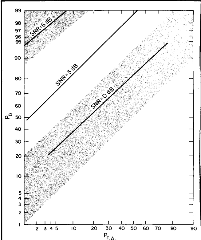
Fig. 16. Receiver operating characteristic curve for trapped-miner receiver.
