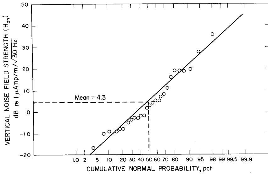
Fig. 7. Statistical distribution of rms surface noise at 630 Hz for a 30-Hz bandwidth.
