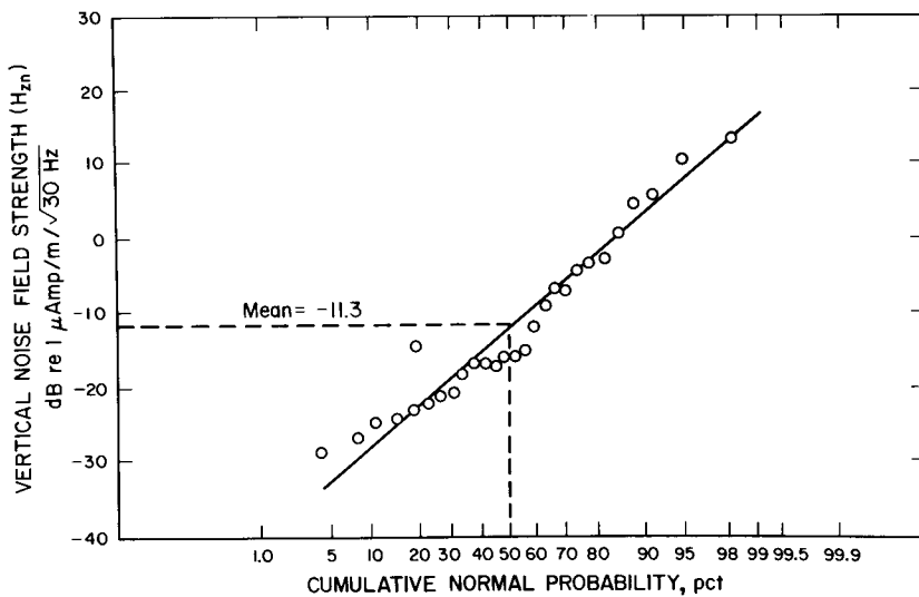
Fig. 9. Statistical distribution of rms surface noise at 1950 Hz for a 30-Hz bandwidth.
