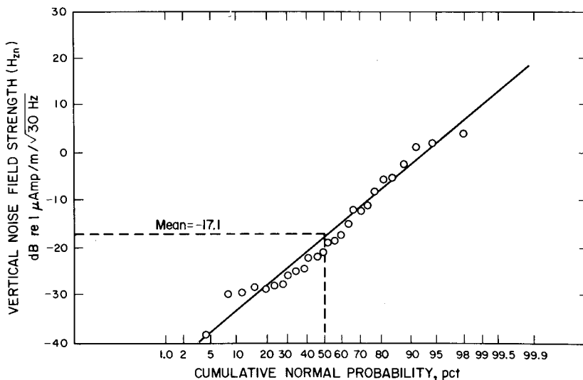
Fig. 10. Statistical distribution of rms surface noise at 3030 Hz for a 30-Hz bandwidth.
