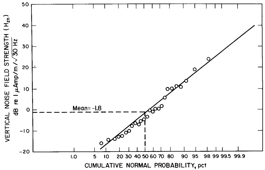
Fig. 8. Statistical distribution of rms surface noise at 1050 Hz for a 30-Hz bandwidth.
