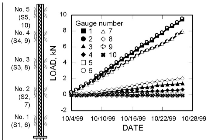
Figure 10.—Load on bolt 4 at Getchell Mine.
