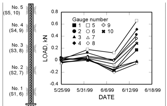
Figure 11.—Load on bolt 14 at K-2 Mine.
