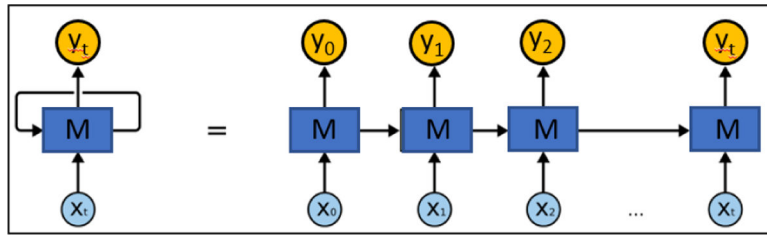
Fig. 3. An unrolled or unfolded RNN
