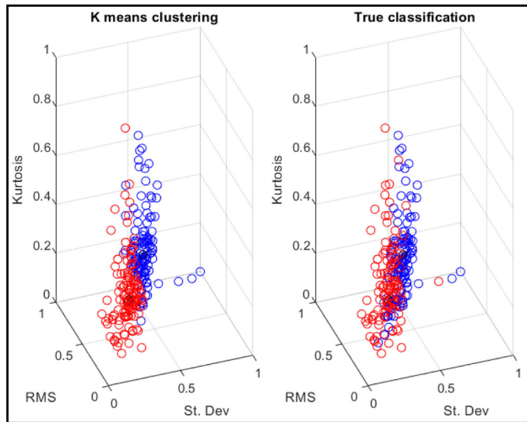
Fig. 6. The graph on the left shows the results of the k means cluster, and the graph on the right shows the true classification.
