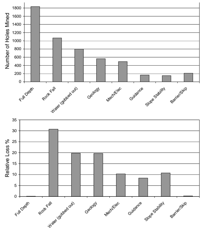
Figure 13. Loss category analysis of 5,289 highwall mining holes (top) and relative losses versus loss categories-3,192,000 planned ft. and 632,000 loss ft (bottom).
