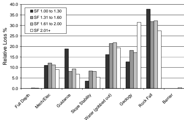
Figure 14. Relative losses as function of loss category and stability factor.
