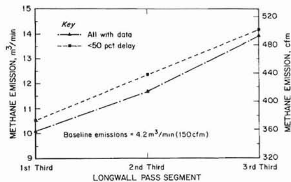
Figure 9. Average methane emissions by pass segment for all bases, VP-3 Mine.
