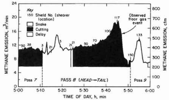
Figure 5. Methane emissions during floor gas event, pass 8, day 2, VP-1 Mine.
