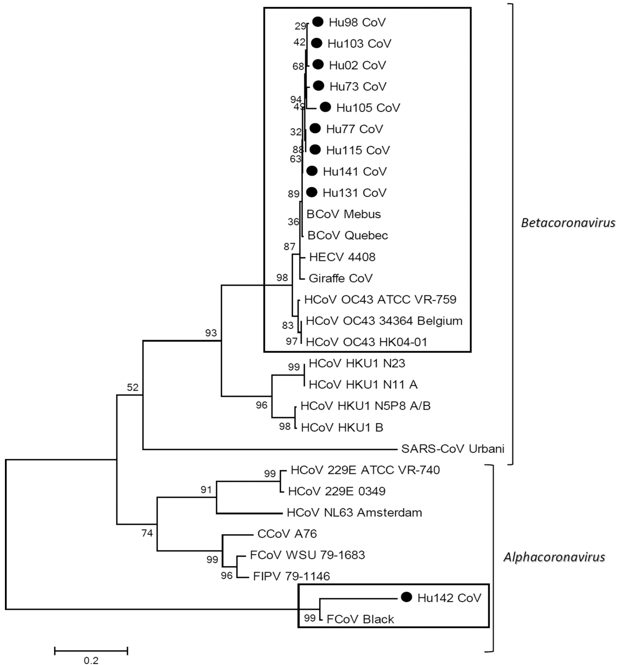
Figure 2. Phylogenetic dendrogram of the partial (460 bp) sequence of the Spike region. The evolutionary history was inferred using the Neighbor-Joining method [32]. The percentages of replicate trees in which the associated taxa clustered together in the bootstrap test (1000 replicates) are shown next to the branches [33]. The tree is drawn to scale, with branch lengths in the same units as those of the evolutionary distances used to infer the phylogenetic tree. The evolutionary distances were computed using the Maximum Composite Likelihood
