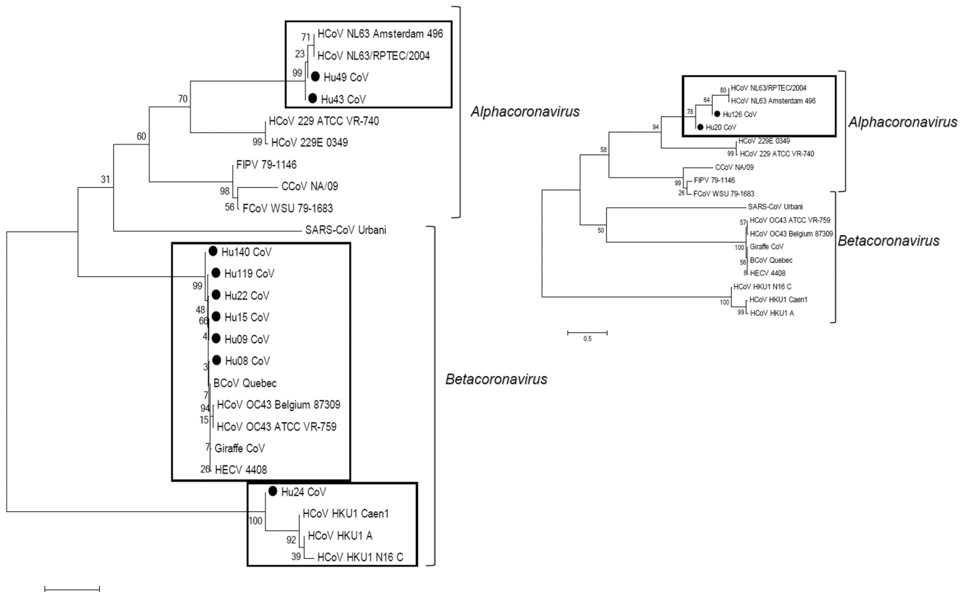
Figure 3. Phylogenetic dendrogram of the partial (460 bp) sequence of the nucleocapsid region. Because only 100–140 bp fragments were obtained for Hu20&126 samples, they were analyzed separately and are shown on a smaller subtree. The evolutionary history was inferred using the Neighbor-Joining method [32]. The percentages of replicate trees in which the associated taxa clustered together in the bootstrap test (1000 replicates) are shown next to the branches [33]. The tree is drawn to scale, with branch lengths in the same units as those of the evolutionary distances used to infer the phylogenetic tree. The evolutionary distances were computed using the Maximum Composite Likelihood method [34] and are in the units of the number of base substitutions per site. Evolutionary analyses were conducted in MEGA5 [25]. ● denotes samples from this study.
