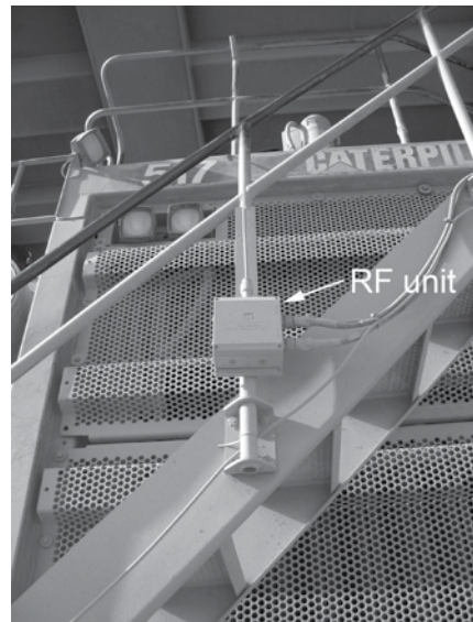
Figure 14. AMT RF unit mounted on the front of a haul truck.
