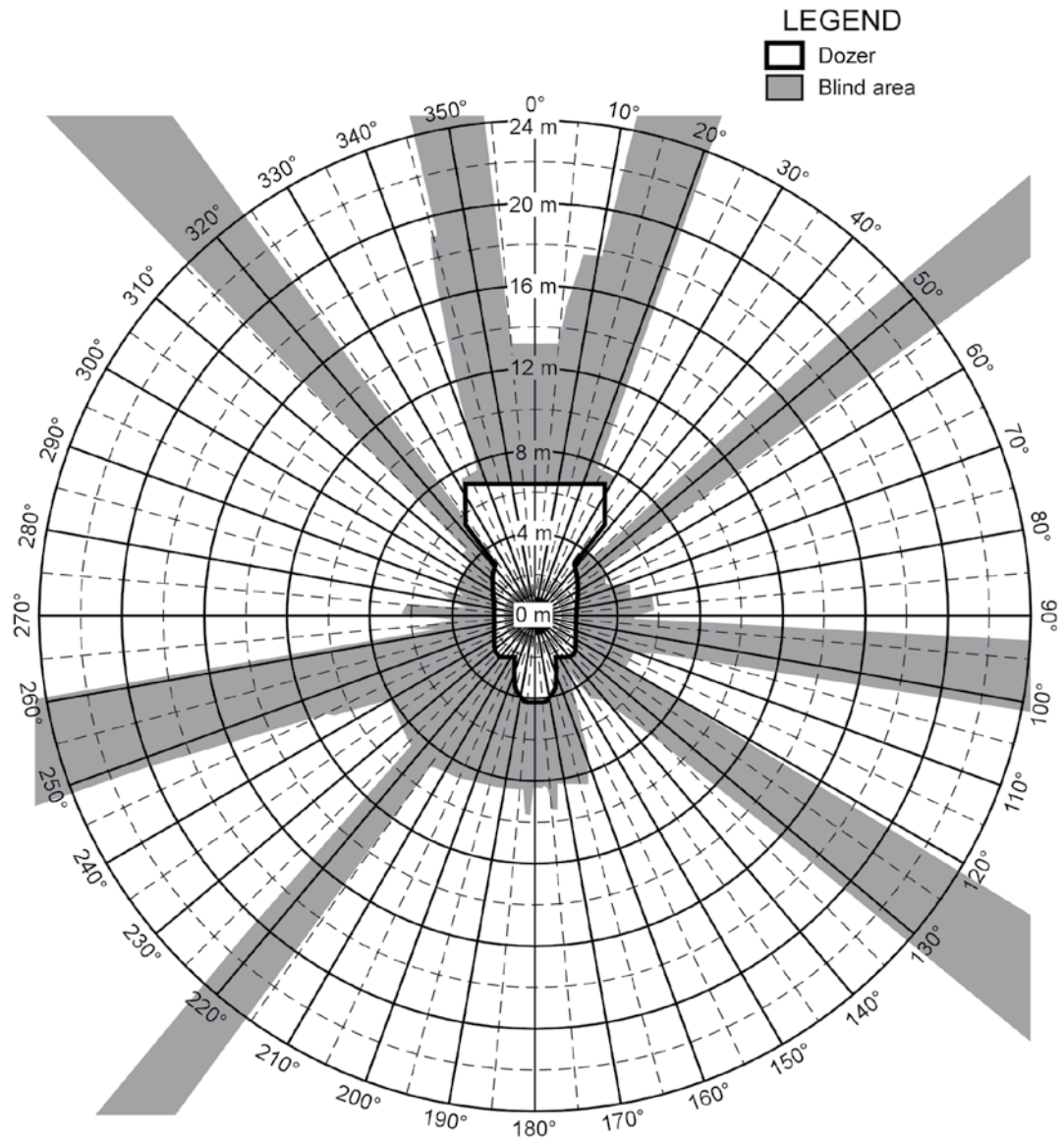
Figure A.12. Blind area diagram for a Caterpillar D11R dozer (1.5 meter plane).
