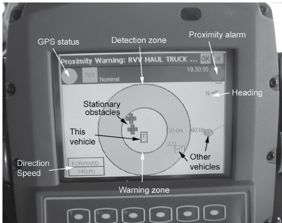
Figure 21. Operator's display for a GPS-based proximity warning system.
