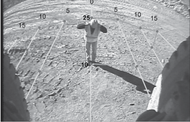
Figure 9. Rear radar detection area as seen from the video monitor (distances in ft).
