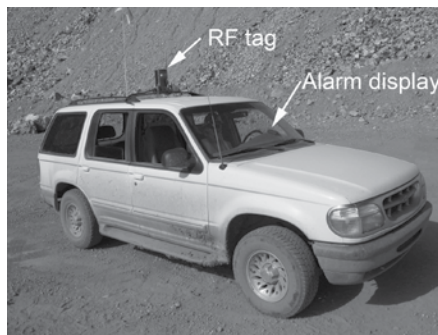
Figure 15. AMT RF tag mounted on a passenger vehicle.
