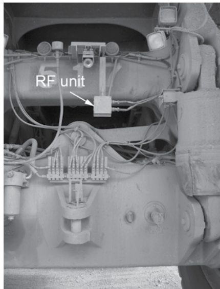
Figure 13. AMT RF unit mounted on the rear of a haul truck.
