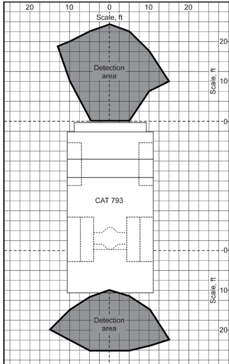
Figure 8. Precognition radar detection areas for a person.
