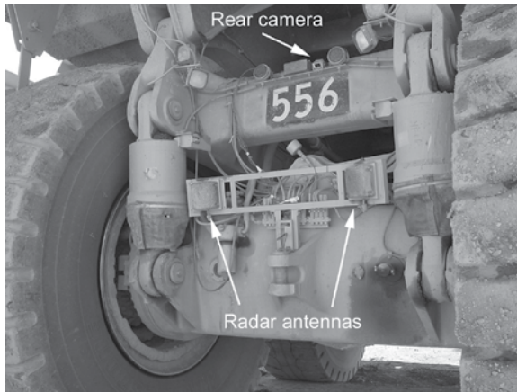
Figure 5. Preco radar antennas and Vision Techniques camera mounted on the rear of a haul truck.
