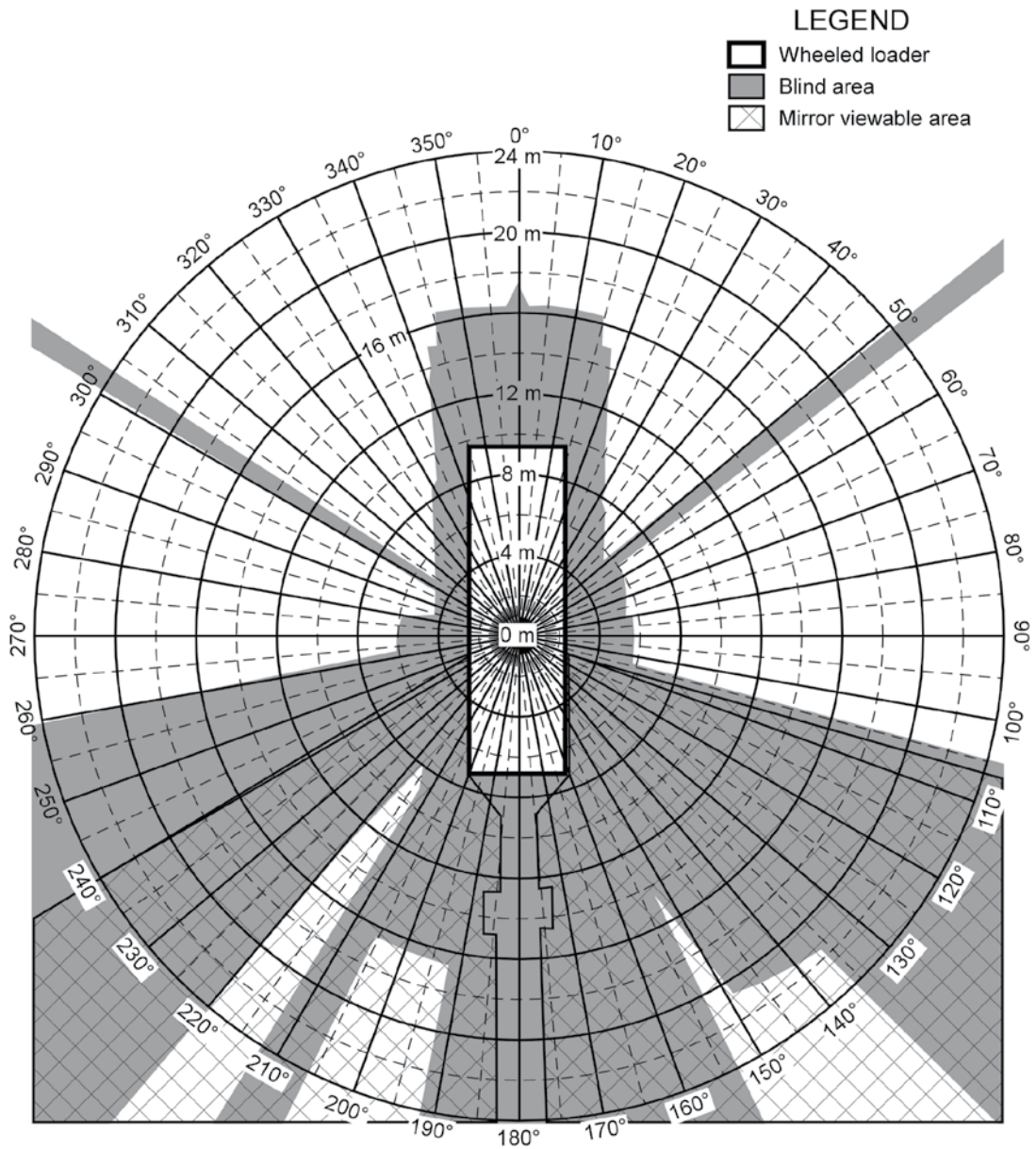
Figure A.5. Blind area diagram for a Caterpillar 992G front-end loader (ground plane).
