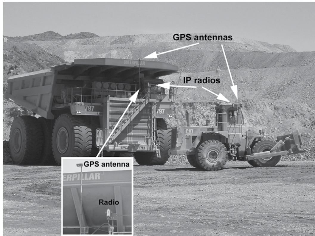
Figure 22. Tests of a GPS-based proximity warning system.
