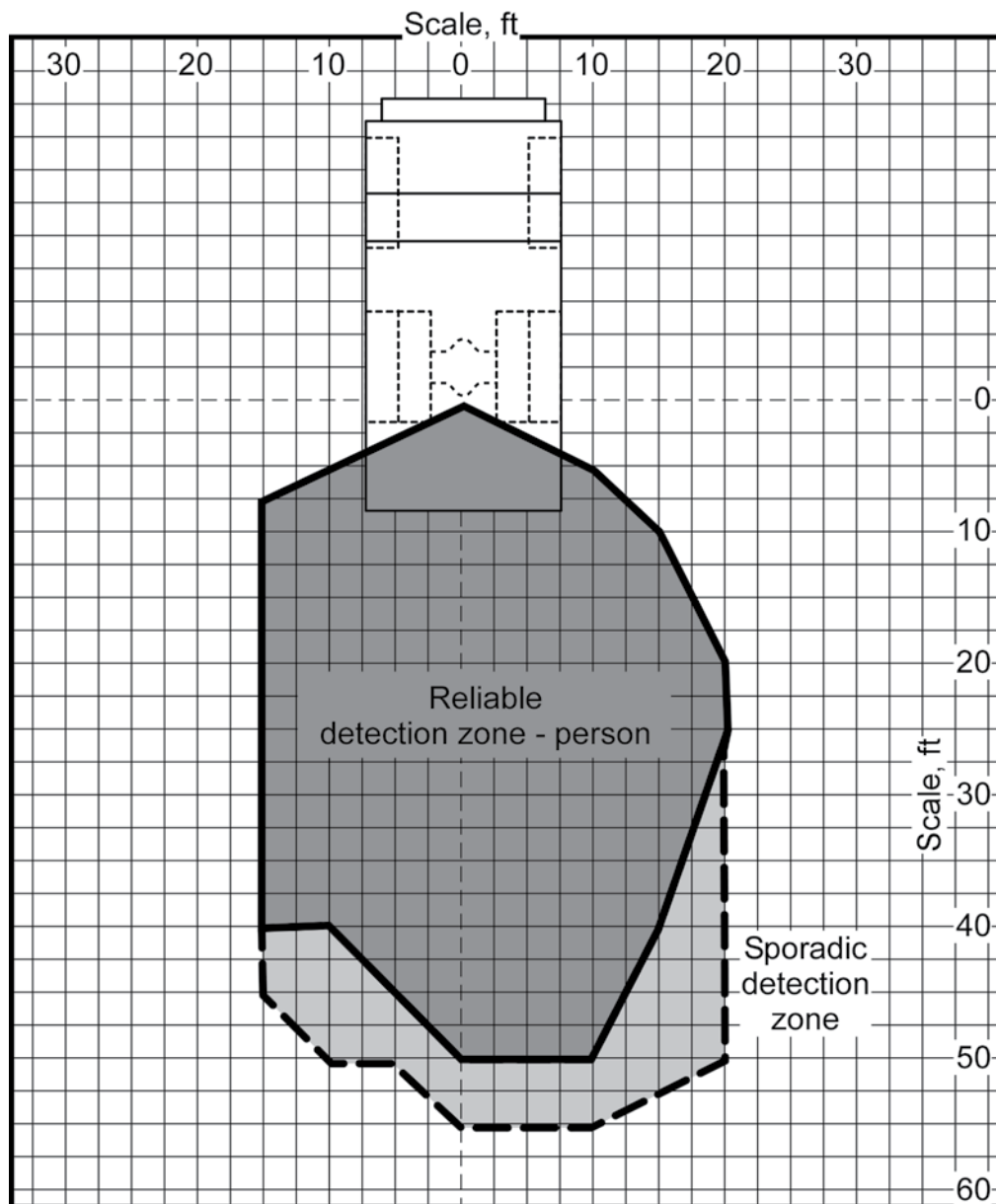
Figure 19. UWB radar detection zone for a person.
