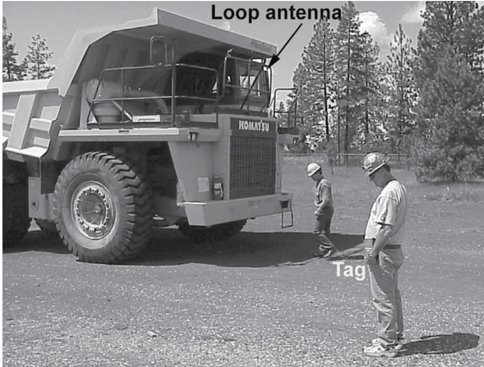
Figure 26. Early version of the Nautilus Buddy tag-based system.
