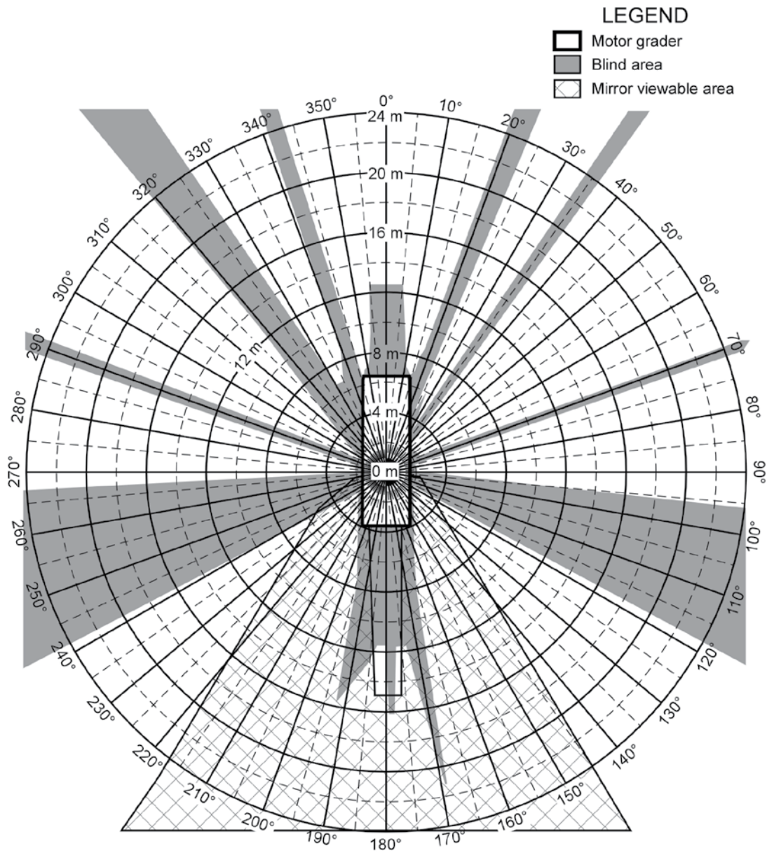
Figure A.15. Blind area diagram for a Caterpillar 16G motor grader (1.5 meter plane).
