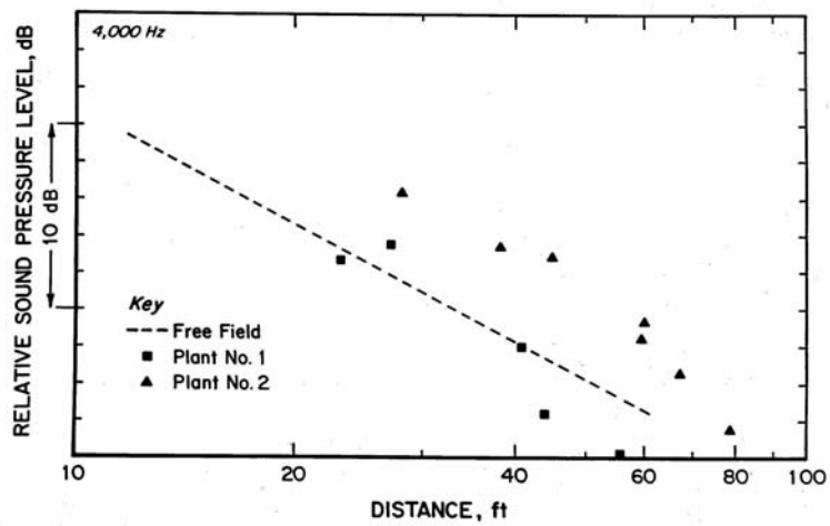
Figure 5.—Sound pressure levels versus distance in structure Nos. 1 and 2.
