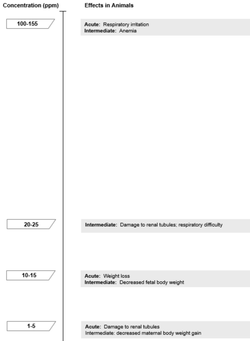
Figure 1-1. Health Effects Found in Animals Following Inhalation Exposure to Hexachlorobutadiene
