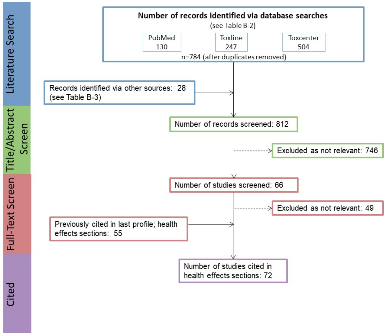
Figure B-1. March 2017 Literature Search Results and Screen for Hexachlorobutadiene
