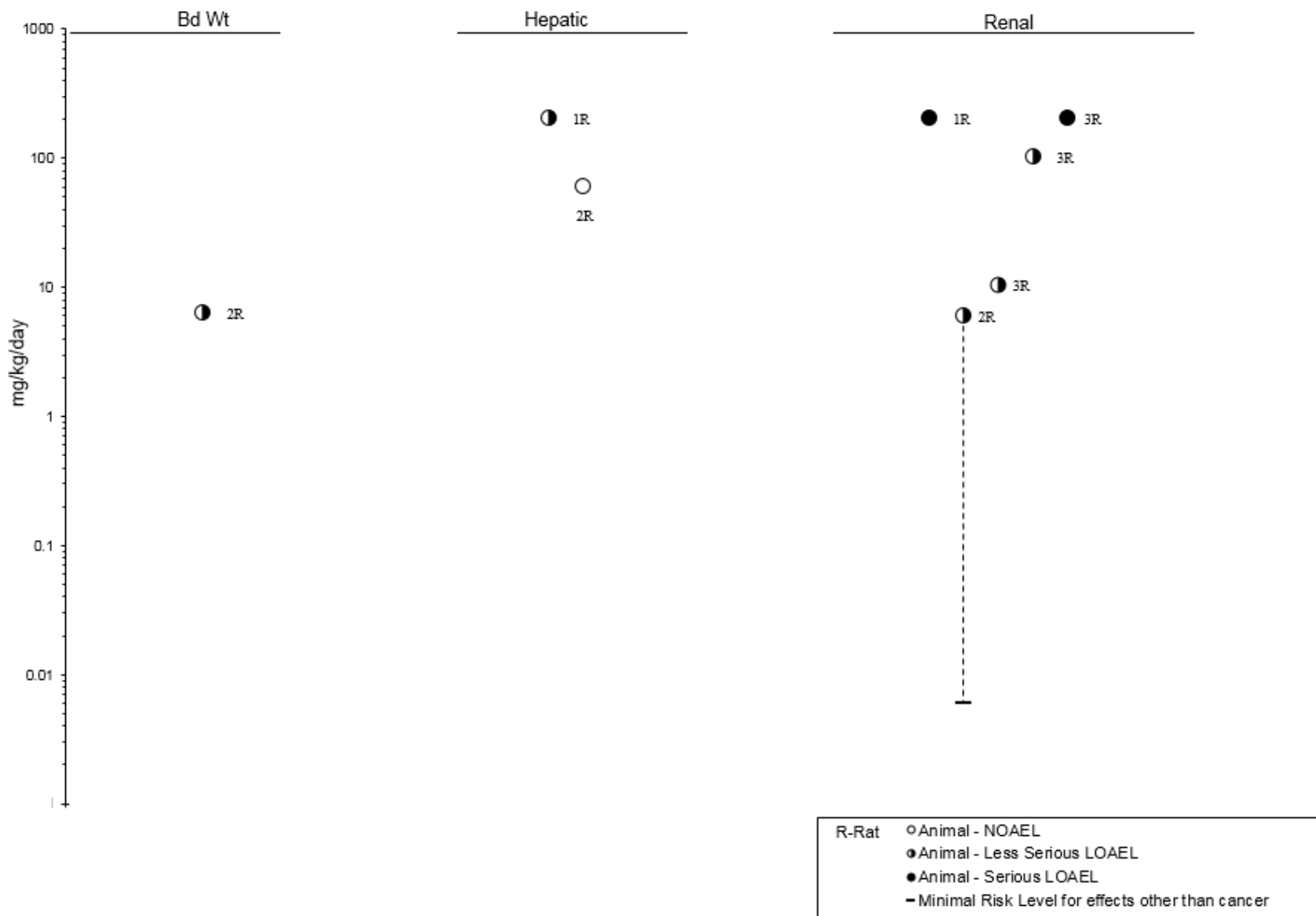
Figure 2-3. Levels of Significant Exposure to Hexachlorobutadiene – Oral Acute (≤14 days)
