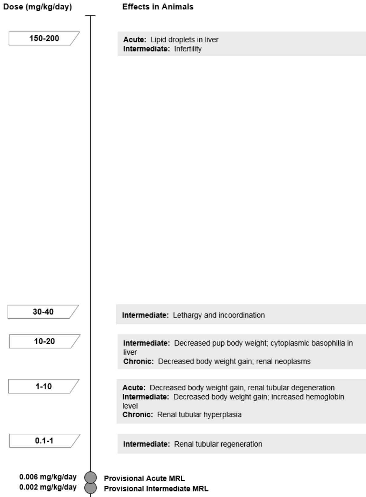
Figure 1-2. Health Effects Found in Animals Following Oral Exposure to Hexachlorobutadiene
